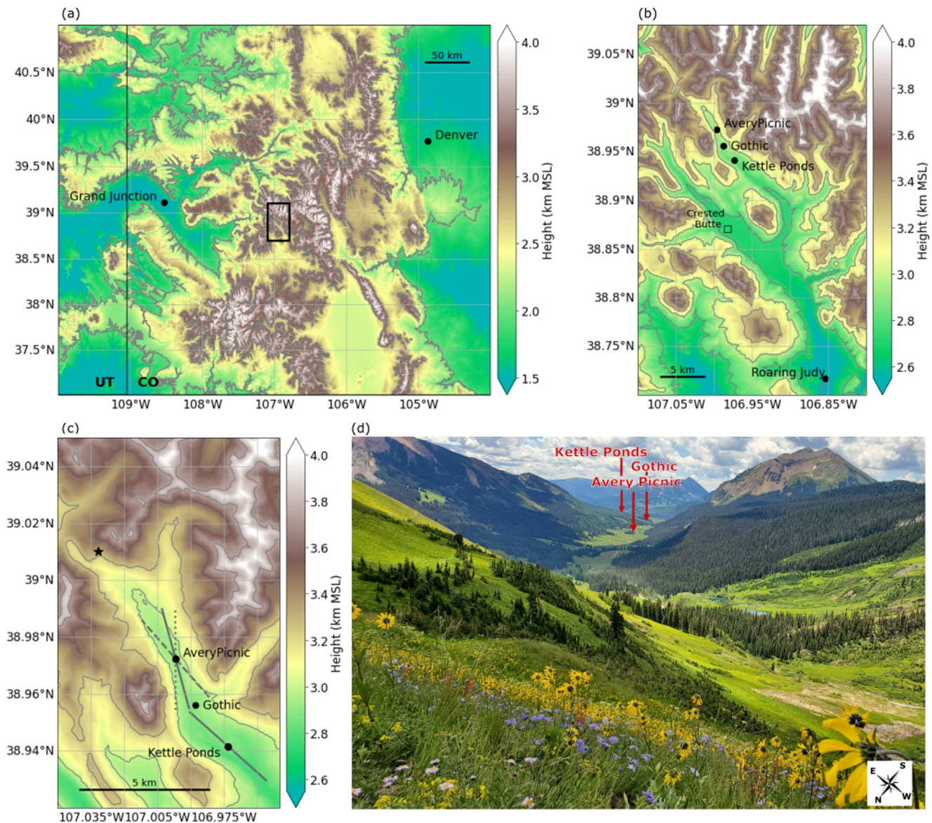
Figure 2. Terrain height based on 30-m resolution elevation data from the Shuttle Radar Topography Mission of (a) the Rocky Mountains in the western part of Colorado, (b) the investigation area in the East River Valley, and (c) zoomed in on the upper part of the East River Valley. The black rectangle in (a) indicates the location of the investigation area. In (c), the solid gray line at Kettle Ponds marks the mean valley axis determined from near-surface up and downvalley (DV) wind measurements. At Avery Picnic, the three different valley axes are indicated: the dotted line is based on nocturnal DV wind measurements, the solid line is based on daytime upvalley wind measurements, and the dashed line marks a subjective valley axis based on the terrain. (d) Photograph taken by the first author in July 2022 on the slope in the upper part of the western fork (location indicated by the star in (c)) looking DV.
