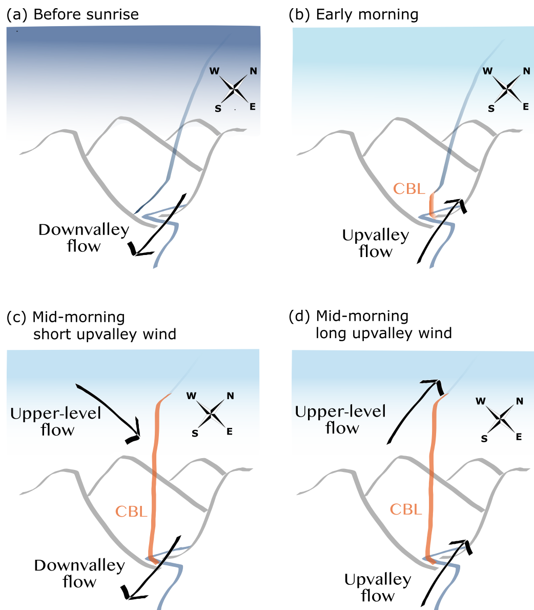
Figure 12. Graphical overview of the flow patterns in the upper East River Valley on days during the warm season when a thermally driven flow system is present in the morning. (a) Before sunrise, a nocturnal surface inversion and downvalley (DV) flow are present. (b) With the development of a convective boundary layer (CBL), the surface inversion is eroded and thermally driven upvalley (UV) wind starts. When the CBL grows above ridge height in midmorning, upper-level momentum is downward transported in the valley and channeled in (c) DV direction when the upper-level flow is southwesterly to northerly (short UV wind day) or in (d) UV direction when the upper-level flow has a southerly component (long UV wind day).
