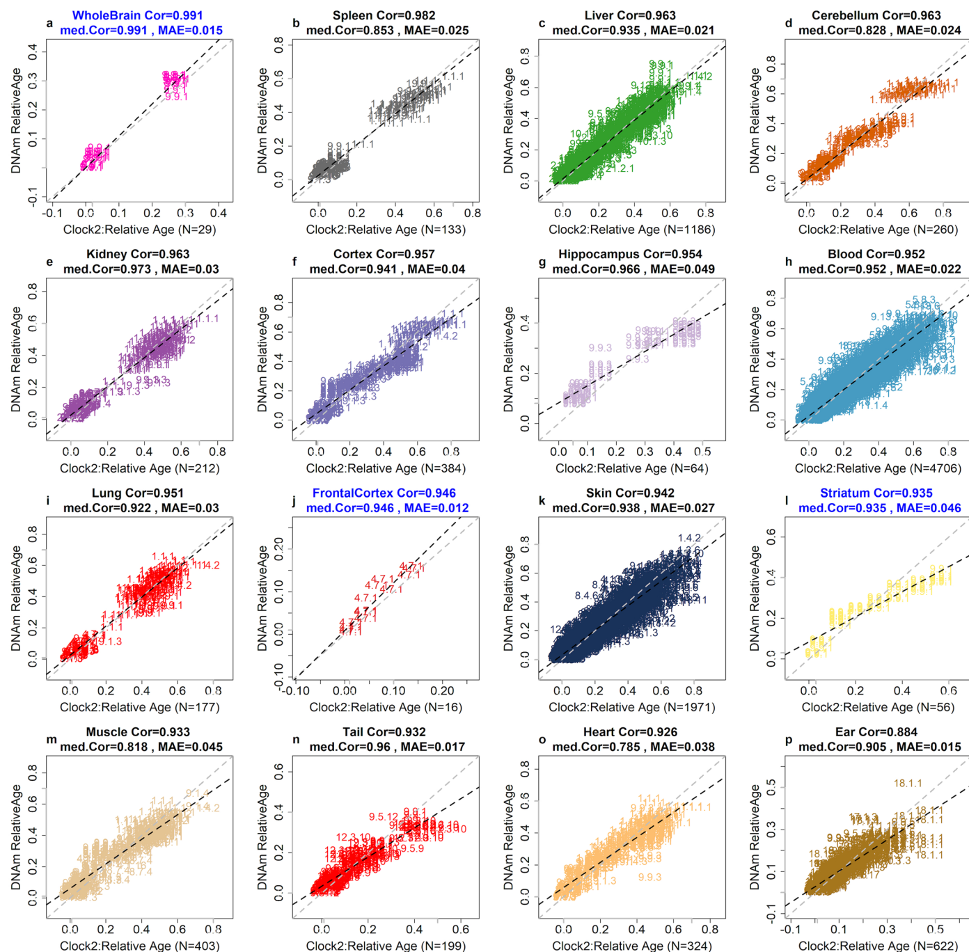
Extended Data Fig. 5 | Universal clock for relative age applied to specific tissues. a–p , DNA methylation-based estimates of relative age (y-axis) versus actual relative age (x-axis). The specific tissue or cell type is reported in the title of each panel. Each sample is labeled by mammalian species index and colored by tissue type (Supplementary Data 1.3–1.4). The analysis is restricted to tissues that have at least 15 samples available. Leave-one-fraction-out cross-validation
