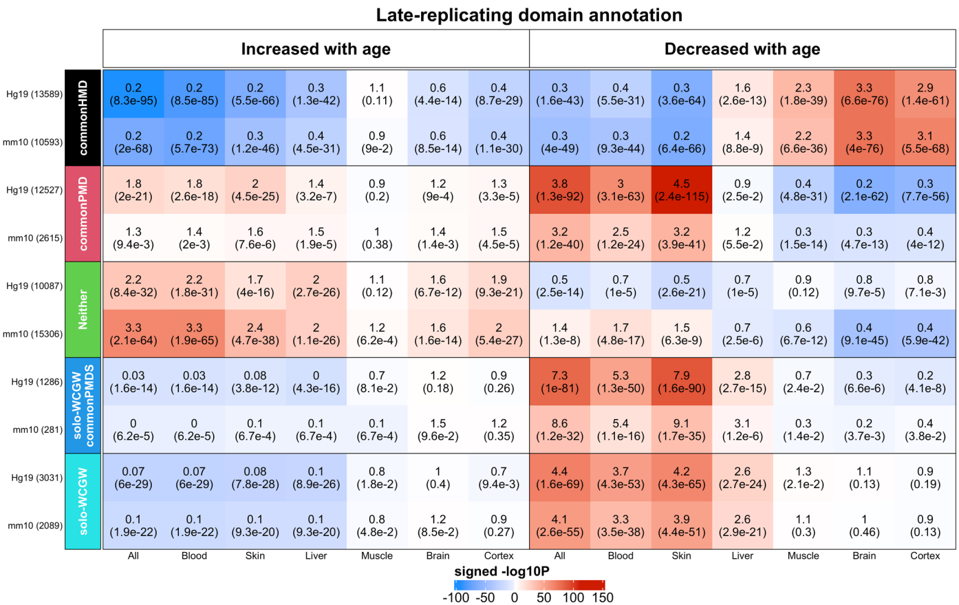
Extended Data Fig. 8 | Overlap with late-replicating domains. The heatmap color-codes the hypergeometric overlap analysis between age-related CpGs (columns) and CpGs related to late-replicating domains in hg19 and mm10 assembly 50 , respectively. Two groups of late-replicating domains were analyzed (1) common PMD/HMD structures: highly methylated domains (commonHMD), partially methylated domains (commonPMD), and neither (Neither), and (2) solo-WCGW structures: genome-wide (solo-WCGW) and those in the common PMD regions (solo-WCGW commonPMDs). The y-axis lists categories of late-replicating domains and number of mammalian array CpGs inside parentheses
