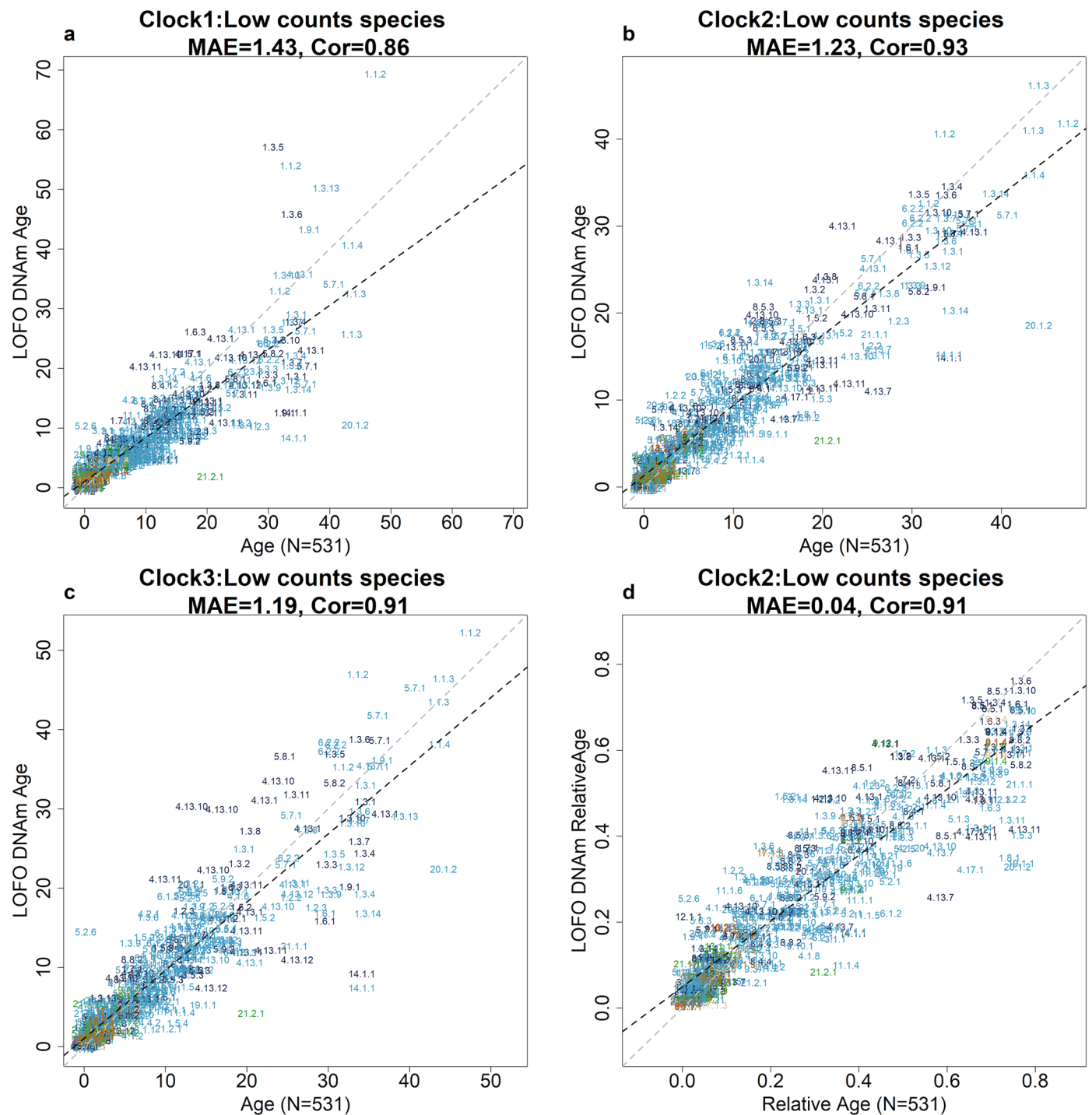
Extended Data Fig. 3 | Universal clocks applied to species with fewer than 15 samples. The title of each panel lists the type of universal clock: a , Clock 1 = basic universal clock based on \log(\text{Age} + 2) , b , d , Clock 2 = universal clock for relative age, c , Clock 3 = universal clock for log-linear age. Leave-one-fraction-out
