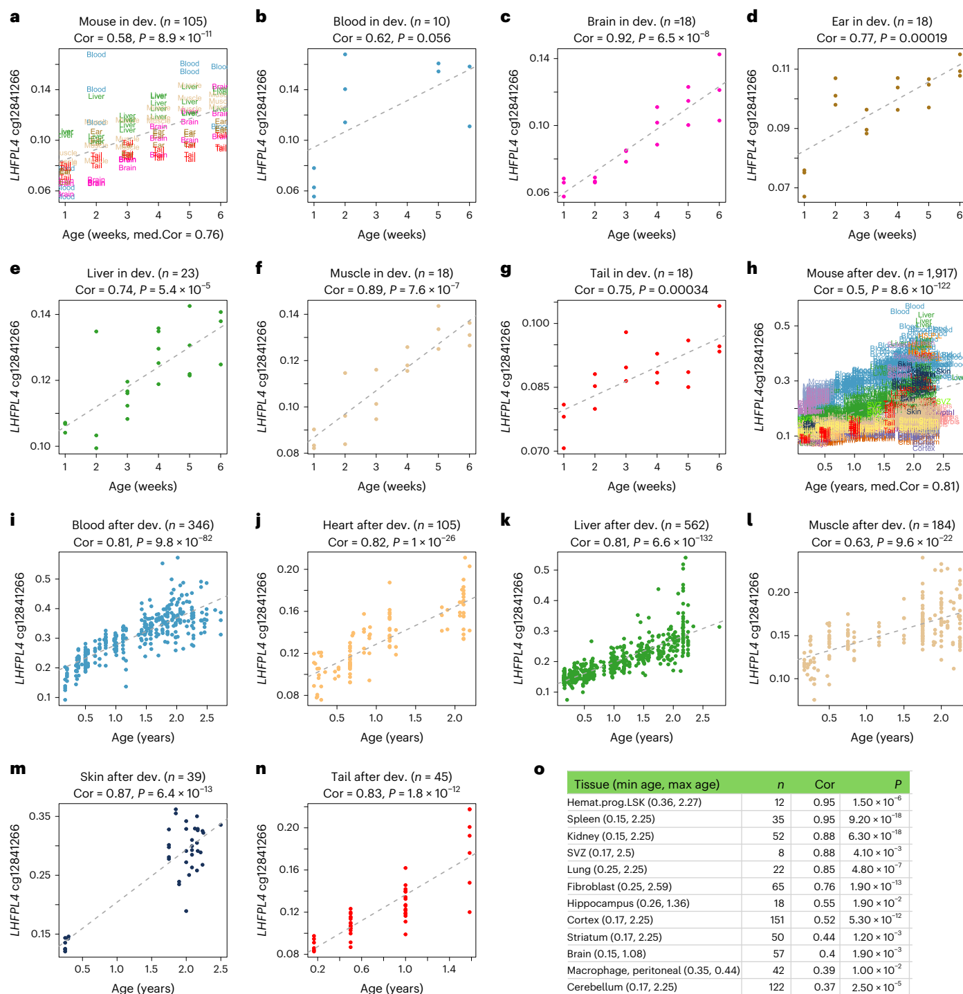
Fig. 5 | Methylation levels of cg12841266 ( LHFPL4 ) versus chronological age in mouse tissues. Results are reported for different tissues and age groups. a–g , Postnatal development (dev.) (from 1 week to 6 weeks). h–o , Age effects in adult mice. Mean \pm s.d. 96 of chronological age is 3.5 \pm 1.7 (1.0–6.0) weeks in the developmental age group and 1.12 \pm 0.72 (0.15–2.78) years in the post-developmental group. a, h , All tissues combined. Each dot (sample) is colored
