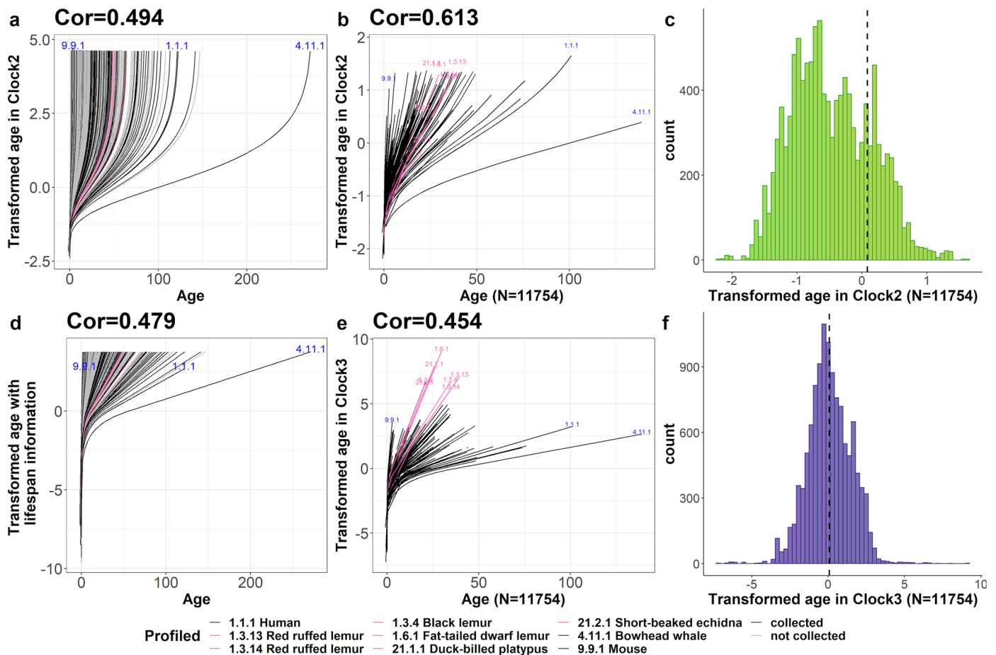
Extended Data Fig. 1 | Transformed age in universal clocks. The plot displays transformed age in universal Clock 2 (a–c) and universal Clock 3 (d–f). (a, b) Loglog transformation of Relative Age (y-axis) versus age in universal Clock 2 and (d, e) log-linear age (y-axis) versus age in our universal Clock 3. Of the 969 mammalian species with available gestation time, age at sexual maturity and maximum lifespan in AnAge database, 339 species are available in our collection. We multiplied the reported maximum lifespan of non-human or non-mouse species by 1.3. Transformed ages were calculated for all the 969 species with simulated age ranging from gestation time through the modified maximum lifespan. The columns (a, d) display all the 969 species with the simulated ages. In panel d, we proposed the log-linear age with the parameter m formulated with maximum lifespan as the information is available for all species ( m = c_1 * \frac{\text{MaxLifespan} + \text{GestationT}}{\text{ASM} + \text{GestationT}} in Methods). Of the 339 species, 185 species with age
