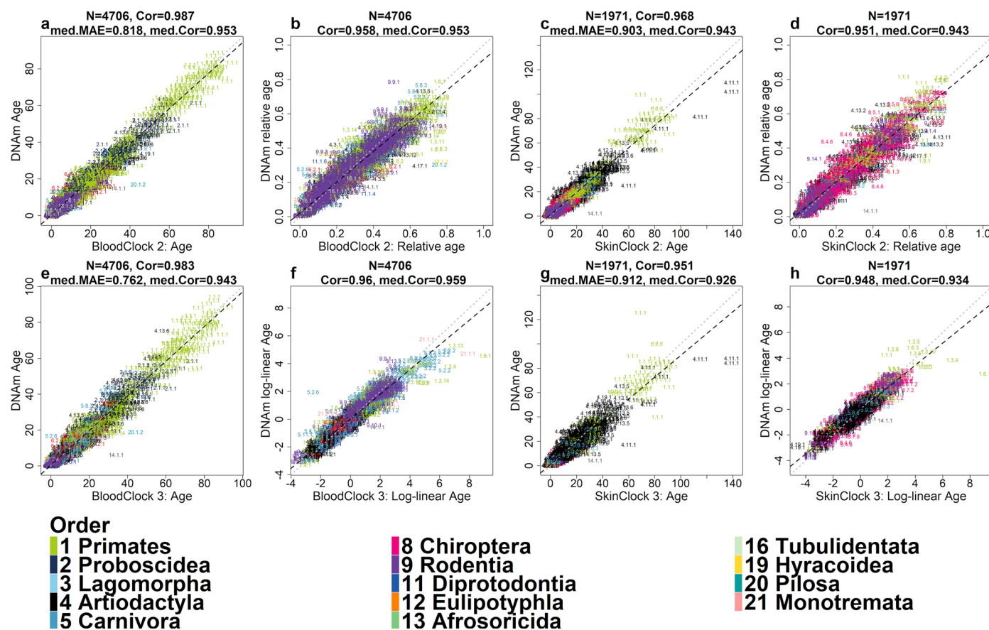
Extended Data Fig. 4 | Universal clocks for specific tissues (blood, skin). These tissue-specific universal clocks were constructed in an analogous fashion to the pan-tissue clocks described in the main text. The panels show leave-one-fraction-out (LOFO) estimates (y-axis) of four clocks: universal blood clock 2 (Universal BloodClock 2) which estimates relative age, universal blood clock 3 (Universal BloodClock 3) which estimates log-linear transformation of age. Analogously, we defined Universal SkinClock2 and Universal SkinClock3. Relative age estimation incorporates maximum lifespan and gestational age and assumes values between 0 and 1. Log-linear age is formulated with age at sexual maturity and gestational
