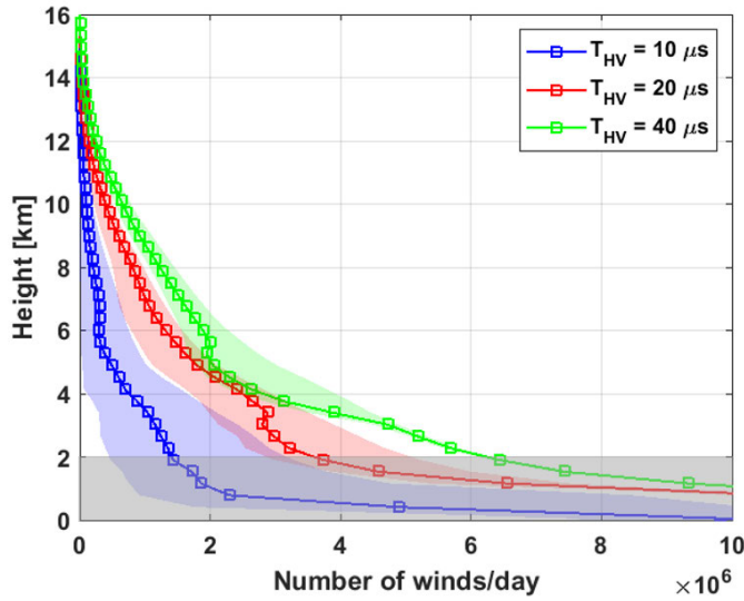
Fig. 9. Profile of the number of 5-km averaged winds better than 1 m/s for different T_{HV} under distinct ghost signal scenarios. The continuous lines indicate the case with normal LDR condition, while the shading spans each line from the 10-dB LDR enhancement and the no-ghost condition. The gray shading corresponds to the ground clutter.
