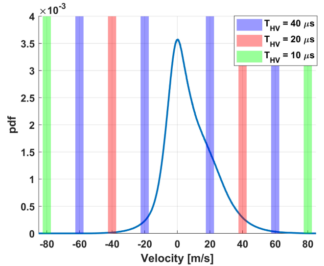
Fig. 10. Expected pdf of WIVERN LOS Doppler velocities (for azimuthal angles between 0^\circ and 180^\circ ) with the regions where biases may occur color-coded according to three different T_{HV} selections.
