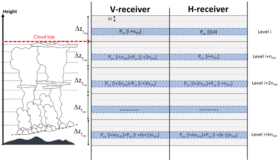
Fig. 3. WIVERN H and V reflectivity profiles separated into different layers separated by \Delta r_{THV} in range and by \Delta z_{THV} in height. Each layer has n_{HV} levels (here only four just for illustrative purposes). The subscripts co and cx indicate copolar and cross-polar signals, respectively. Here, H is the leading pulse.
