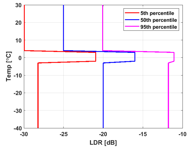
Fig. 14. Simulated LDR profiles at the fifth, 50th, and 95th percentiles.
