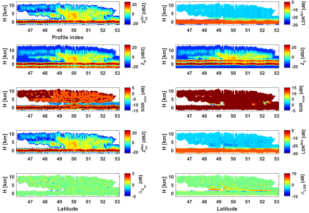
Fig. 5. Performance of the retrieval on a scene extracted from the CloudSat orbit: 2007-018-230022-03868. (Top row) True copolar reflectivity and LDR; (second row) received leading pulse and trailing pulse reflectivity; (third row) \text{SGR}_{\min} with the contour of the std of Doppler LOS winds in the left column and \text{SGR}_{\max} in the right one; (fourth row) retrieved copolar reflectivity and LDR; and (last row) errors in the retrieved copolar reflectivity and LDR (the difference between the original and the retrieved).
