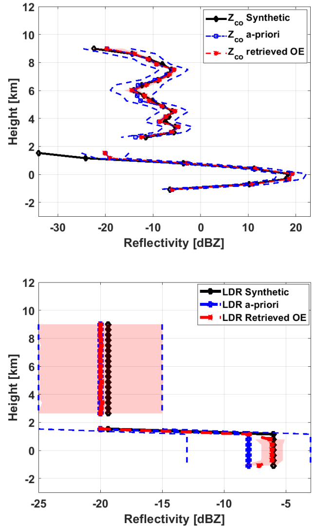
Fig. 4. Retrieved copolar reflectivity (top) and LDR (bottom) for the profile shown in Fig. 2. A priori and synthetic profiles are shown in blue and black color. A 5-km horizontal averaging is considered. The error standard deviation of the OE solution is shaded in red, while the blue dashed lines represent the uncertainty on the a priori.
