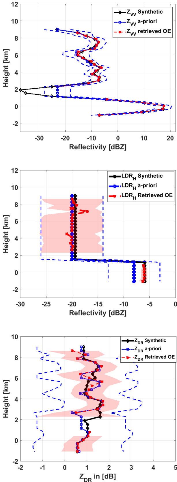
Fig. 11. (Top) Retrieved copolar V reflectivity, (middle) LDR_H , and Z_{DR} for the profile shown in Fig. 2. A priori and synthetic profiles are shown in blue and black color. A 5-km averaging is considered. The error standard deviation of the OE solution is in red, while the blue dashed lines represent the uncertainty on the a priori.
