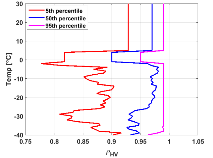
Fig. 13. Simulated \rho_{HV} profiles at the fifth, 50th, and 95th percentiles.
