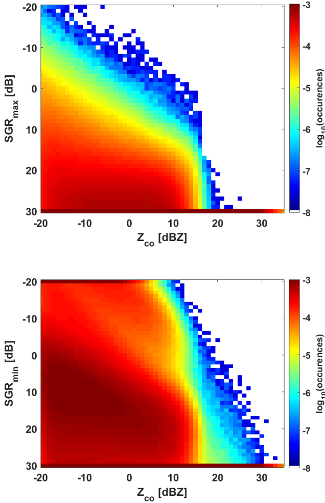
Fig. 6. Absolute frequency of the occurrences of (bottom) “single” and (top) “double” ghosts (with a given strength identified by the SGR value, y-axis) as a function of the copolar reflectivity, x-axis for T_{HV} = 20 \mu s . The binning size is 1 dB for both Z_{co} and SGR. In the first and last rows, all the values exceeding the highest or being lower than the lowest SGR range of values are summed up together.
