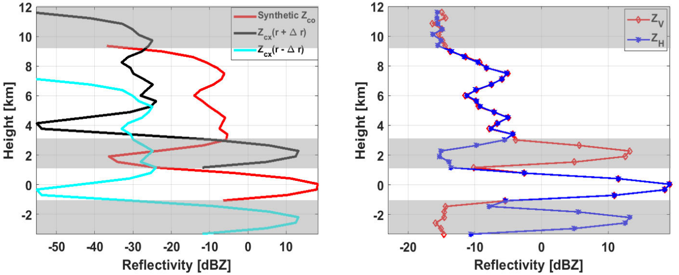
Fig. 2. (Right) Example of simulated WIVERN H and V signals inclusive of noise derived from (left) CloudSat profile. In the left panel, the red line represents the synthetic CloudSat copolar profiles, whereas the black and cyan lines correspond to the cross-polar signal derived by multiplying the copolar signal for climatological LDR profiles and by shifting it by \pm \Delta r_{20} \mu s = 3 km, i.e., a shift \pm \Delta z_{20} \mu s = 2.24 km in height. Areas affected by SGR_{\min} < 0 (i.e., at least one of the crosstalk signals exceeds the copolar signal) are highlighted by gray shading.
