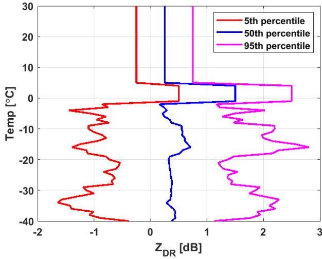
Fig. 12. Simulated Z_{DR} profiles at the fifth, 50th, and 95th percentiles.
