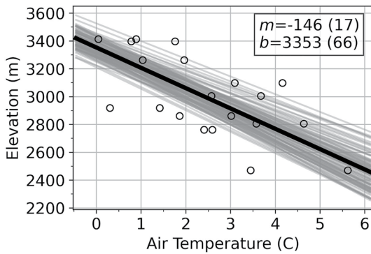
Figure 3. Annual average air temperature versus elevation measured at weather stations and STOTEL sites within the East River Watershed for the years 2019 and 2020. The thick black line corresponds to the mean linear lapse rate and the gray lines are random realizations from the slope ( m ) and intercept ( b ) posterior distributions. Values in parentheses are 1 standard deviation in the best fit parameters.
