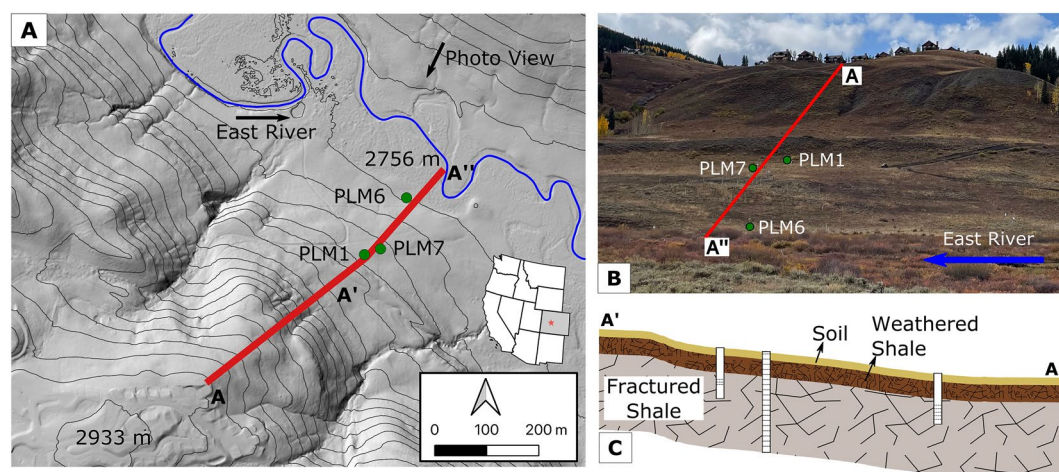
Figure 1. (a) Elevation contour map and (b) image of the study site located in East River Watershed near Crested Butte, Colorado. The red line indicates the Pumpphouse lower montane (PLM) hillslope transect and the green dots are the locations of the three observation wells. (c) Simplified cross section along the bottom portion of the PLM hillslope transect showing well positions and screened intervals.
