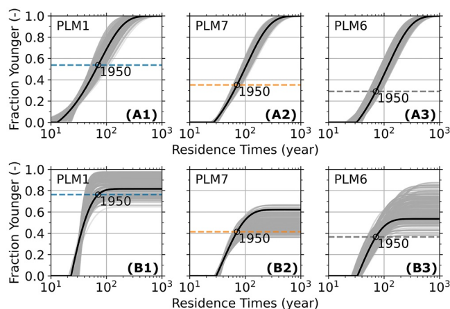
Figure 12. Groundwater residence time cumulative density distributions assuming (a) the exponential piston-flow model (EPM) residence time distribution (RTD) and (b) the binary mixing EPM–piston-flow model (PFM) RTD. The solid black curve is the average distribution of residence times and the light gray curves are samples from the posterior distribution. The open circle and corresponding horizontal line corresponds to the fraction of the total sample that is characterized with residence times that are modern (after 1950).
