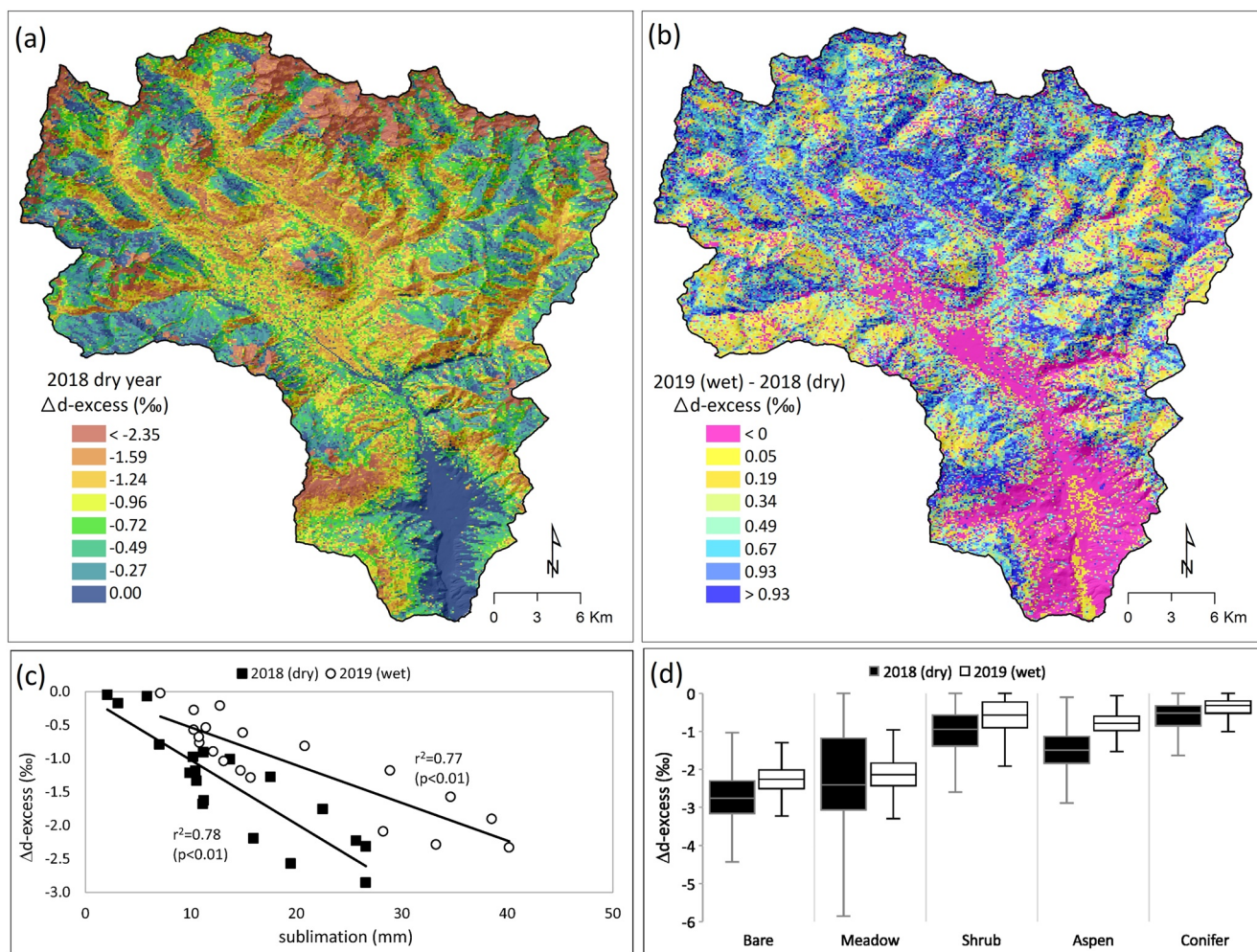
Figure 3. (a) Spatial distribution of snowpack changes to d-excess ( \Delta d\text{-excess} ) due to post-depositional fractionation during 2018, a dry water year. More negative values indicate greater snowpack fractionation. (b) The difference in \Delta d\text{-excess} between 2019 (wet) and 2018 (dry). Positive values indicate a decrease in fractionation in 2019. (c) \Delta d\text{-excess} as a function of sublimation across elevation aggregated at 50 m increments, (d) \Delta d\text{-excess} for various vegetation cover types.
