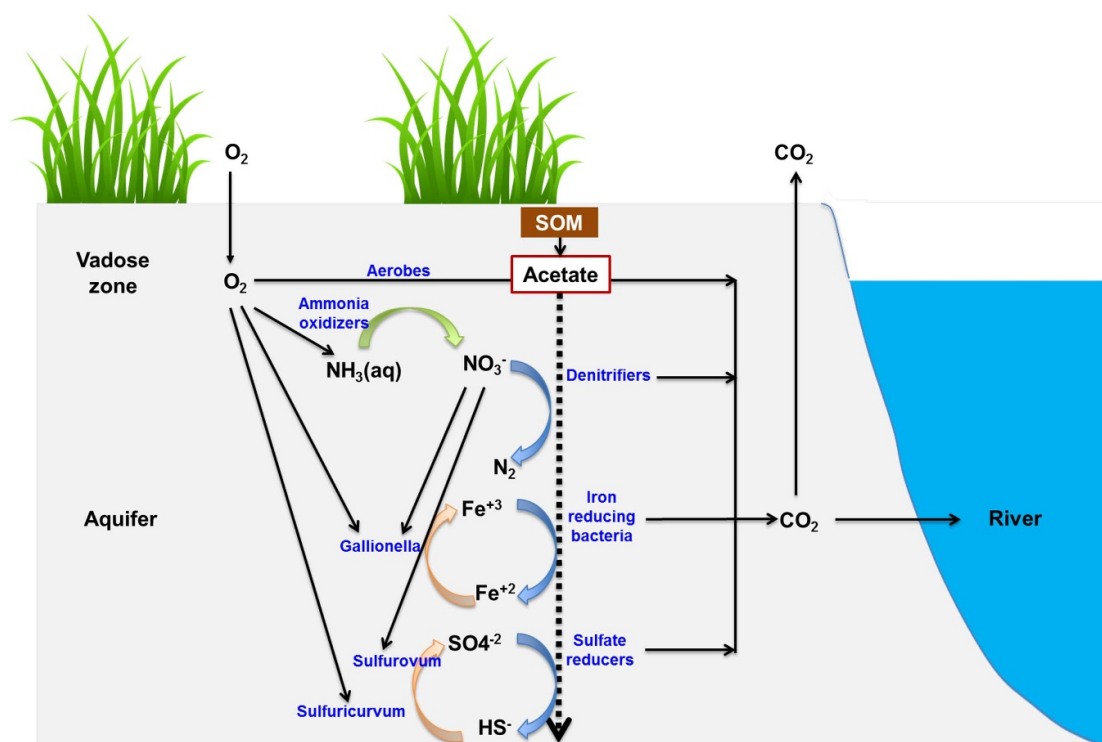
Figure 4. Example of a biogeochemical reaction network used to simulate processes in the Rifle flood plain (from Arora et al 2016b).
