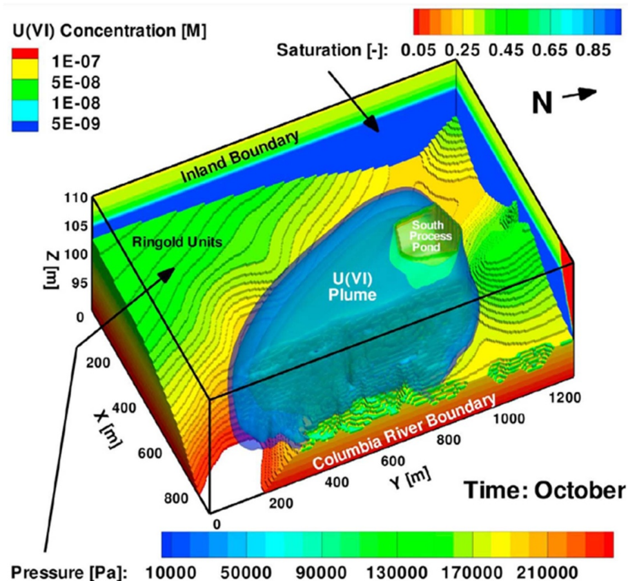
Figure 5. Example of a 3D flow and reactive transport simulation of the Hanford 300 Area, with hydrological and geochemical transients driven by changing water stages in the Columbia River (from Hammond and Lichtner 2010). Hammond and Lichtner (2010). John Wiley & Sons. Copyright 2010 by the American Geophysical Union.
