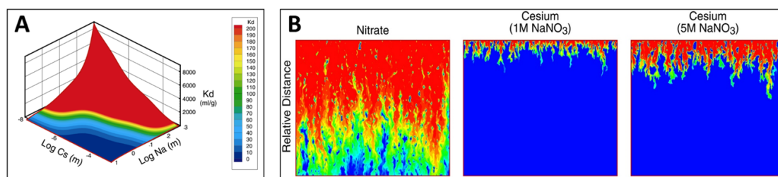
Figure 6. Example of ^{137}\text{Cs} transport in the Hanford 200 Area tank farm. (A) Effective linear distribution coefficient ( K_d ) for \text{Cs}^+ (from Steefel et al 2003). The K_d depends on both the competing cation concentration ( \text{Na}^+ associated with \text{NaNO}_3 in the tank wastes), and on \text{Cs}^+ itself because of the presence of at least two sites with different selectivities for \text{Cs}^+ versus \text{Na}^+ ; (B) Relative migration of nitrate (nonreactive), and \text{Cs}^+ at 1 M \text{NaNO}_3 and 5 M \text{NaNO}_3 . The high \text{Na}^+ concentrations in the tank leak explain the enhanced migration and thus weaker-than-expected retardation of ^{137}\text{Cs} at the Hanford 200 tanks (from Steefel et al 2005).
