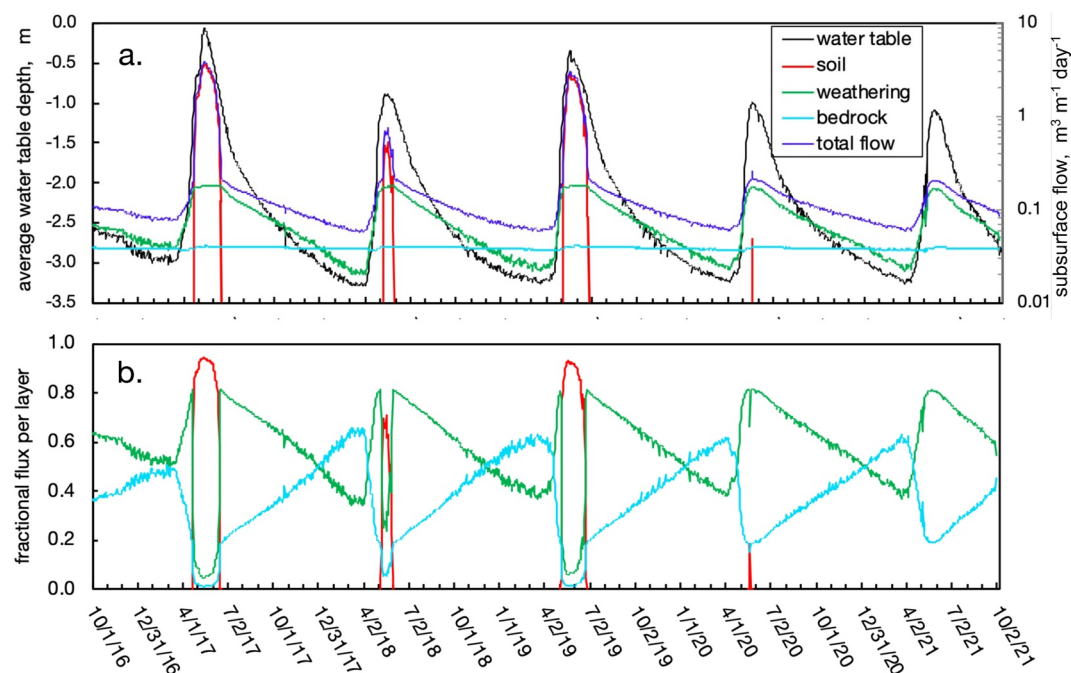
Figure 5. Impacts of annual water table fluctuations on subsurface flow. (a) Annual variations in water table depth and resulting calculated downslope flow along different zones of the hillslope. (b) Time-dependence of fractional contributions of flow along the soil, weathering zone, and fractured bedrock to overall subsurface flow.
