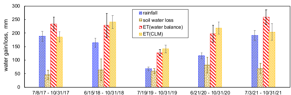
Figure 9. Soil water balance calculations of ET , compared with ET (Community Land Model [CLM]) over summer-fall intervals following cessation of snowmelt drainage. Uncertainties in rainfall and ET (CLM) were estimated as 10% of their respective values, except for the 2021 ET uncertainty which was taken as 15% because its October 2021 ET was estimated from the average of previous Octobers. Uncertainties in soil water losses were assigned to standard errors from values obtained at PLM1, PLM2, and PLM3. Uncertainties in ET (water balance) were estimated as the root mean square uncertainties from summing soil water losses and rainfall.
