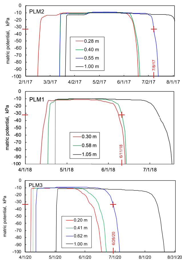
Figure 7. Examples of soil matric potential sensor responses during snowmelt events, illustrating selection of drainage cessation dates when \psi declines below -33 kPa at depths shallower than 1.00 m.
