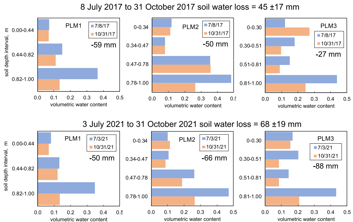
Figure 8. Profiles of volumetric water contents in soils in 2017 and 2021, at cessation of soil drainage (blue), and on October 31. The mm values in each plot indicate soil water losses over the summer to fall intervals.
