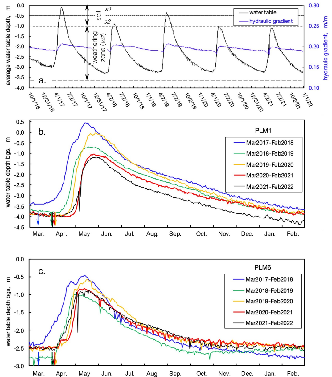
Figure 3. Temporal trends in hillslope water table depth. (a) Average water table depth below the hillslope soil surface and hydraulic gradient between PLM1 and PLM3/6. The water table rises from the weathering zone into the soil zones s_2 and s_1 when snowmelt recharge is high during WY2017 and WY2019. The trend for the drought WY2018 indicates that residual drainage from the unusually high snowmelt from WY2017 supported water table rise into the soil zone despite low 2018 snowmelt. Annual water table depth variations, showing variations in local behavior among different water years at upslope PLM1 (b) and downslope PLM6 (c), respectively. Color-coded arrows along the abscissa indicate times when 5-day average air T began exceeding 0^{\circ}\text{C} .
