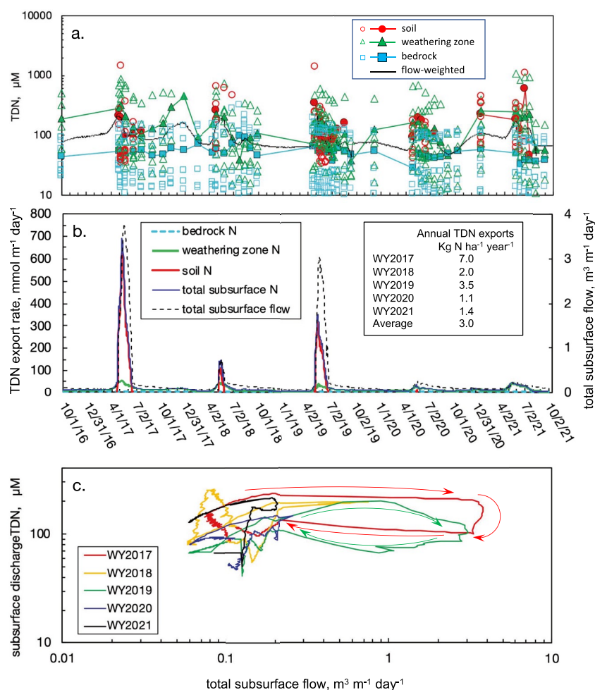
Figure 6. Hillslope subsurface total dissolved nitrogen (TDN) concentrations and transport. (a) Time trends in TDN concentrations in pore waters, (b) calculated TDN export rates along different zones of the hillslope, and (c) subsurface C - Q relations for TDN over five water years.
