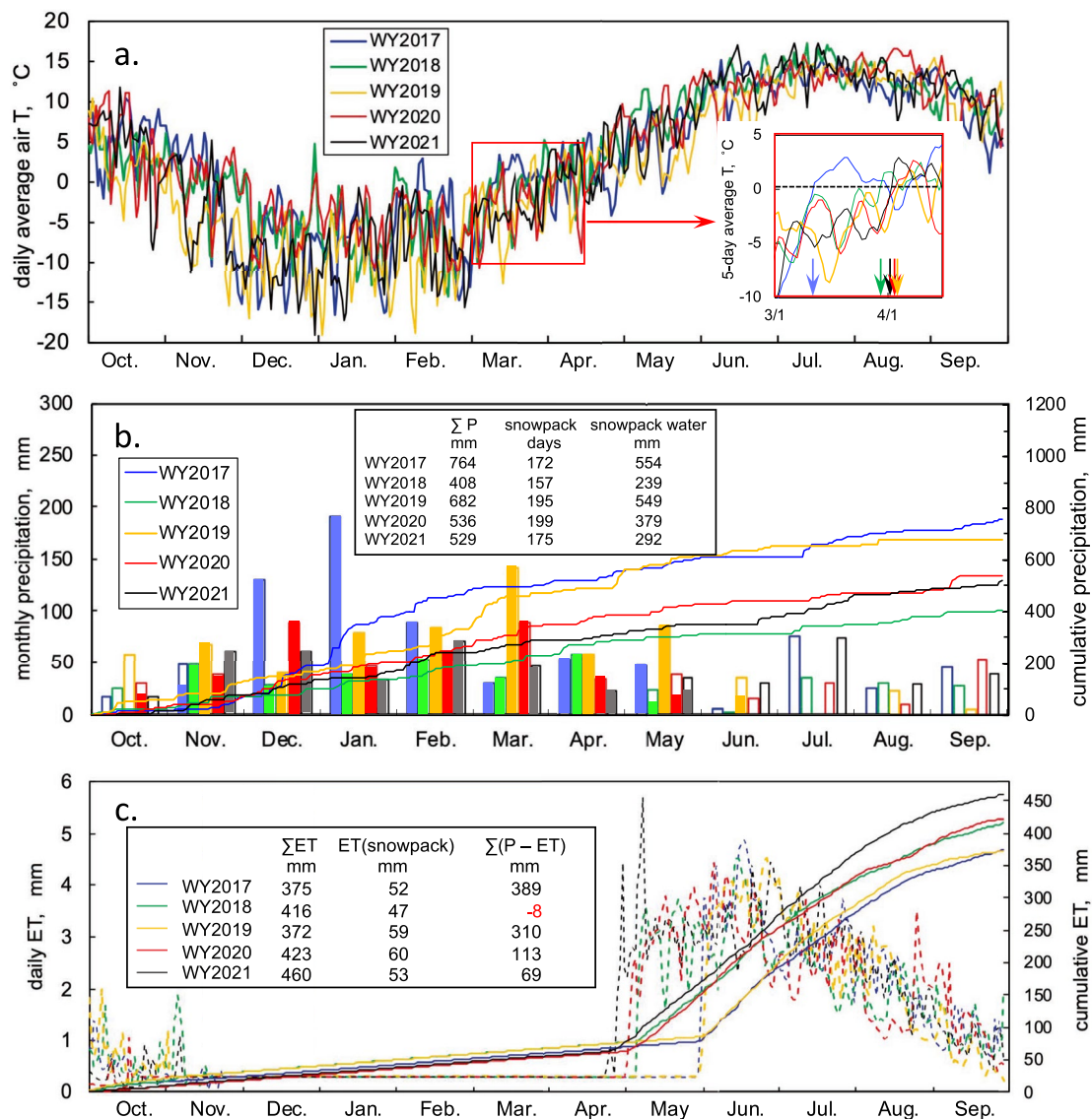
Figure 2. Meteorological conditions at the hillslope site for WY2017–WY2021. (a) Average daily air temperatures. The inset graph shows 5-day running average T during March and April, highlighting the increase above 0°C indicative of snowmelt initiation. Color-coded arrows along the abscissa of the inset graph indicate dates when 5-day average air T began exceeding 0°C. (b) Monthly precipitation (filled = snow, unfilled = rain) and cumulative precipitation. (c) Evapotranspiration calculated with the Community Land Model and an estimated sublimation rate of 0.3 mm day -1 from snow cover.
