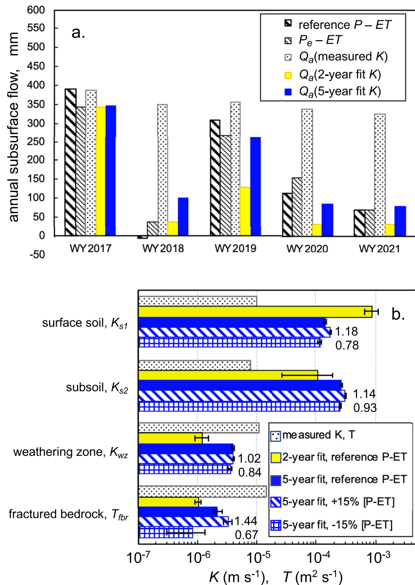
Figure 4. The dependence of calculated annual subsurface flow Q_a on hydraulic properties. (a) Estimates of annual subsurface flow based on P-ET , P_e-ET , transmissivity feedback fluxes using measured K and T_{fb} calibrated to yield total subsurface flow in agreement with P-ET for WY2017, and fitting of hydraulic properties to yield fluxes that best match P_e-ET over five years. (b) Comparisons between average local hydraulic properties obtained from measurements in auger holes and piezometers and fit parameter values obtained by matching annual subsurface flow Q_a to P-ET . The 2-year fits result in a rmsd between P_e-ET and Q_a of 71 mm when applied to all 5 years. Optimizing hydraulic properties over all 5 years reduces this rmsd to 43 mm. Hydraulic properties consistent with \pm 15\% changes in P-ET are also shown. The uncertainty bars span ranges of K and T that yield rmsd that are within 1 mm of rmsd minima. Ratios of optimized K and T relative to their reference values are shown for the \pm 15\% [ P-ET ] cases.
