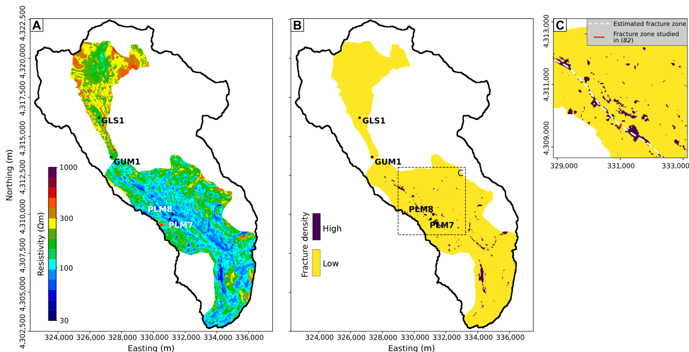
Fig. 9. Predicted shallow subsurface resistivity and fracture density. (A) Resistivity is predicted using an ERT (73) model, using topographic elevation, slope, aspect, and vegetation type as estimators. The variation in resistivity (low resistivity in the lower watershed, high resistivity in the upper watershed) agrees with observational studies (60) showing a higher degree of metamorphism in the upper watershed. (B) Fracture density is defined on the basis of the relationship gained from the borehole data using a resistivity of 70 ohm-m. Linear features showing areas of high fracture density are postulated to correspond to fracture zones. (C) The area of the fracture zone analyzed in (83) lies along the estimated and known fracture zones.
