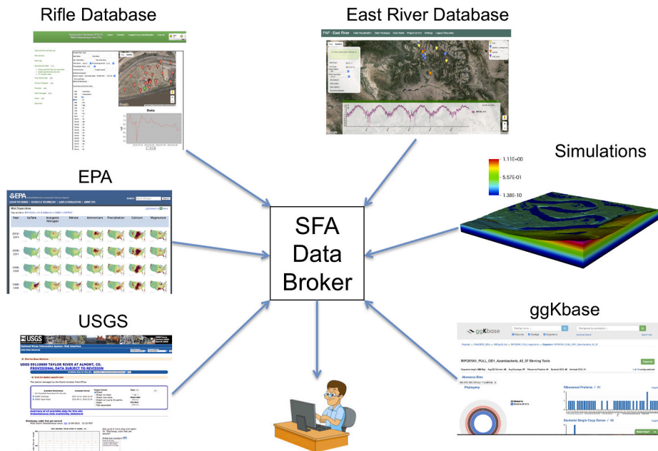
Fig. 5. Conceptual diagram of the functionality desired from the BASIN-3D supported data brokering system for the Watershed Function SFA. The broker would connect to various data sources across organizations and present an integrated view of the data to the user.
