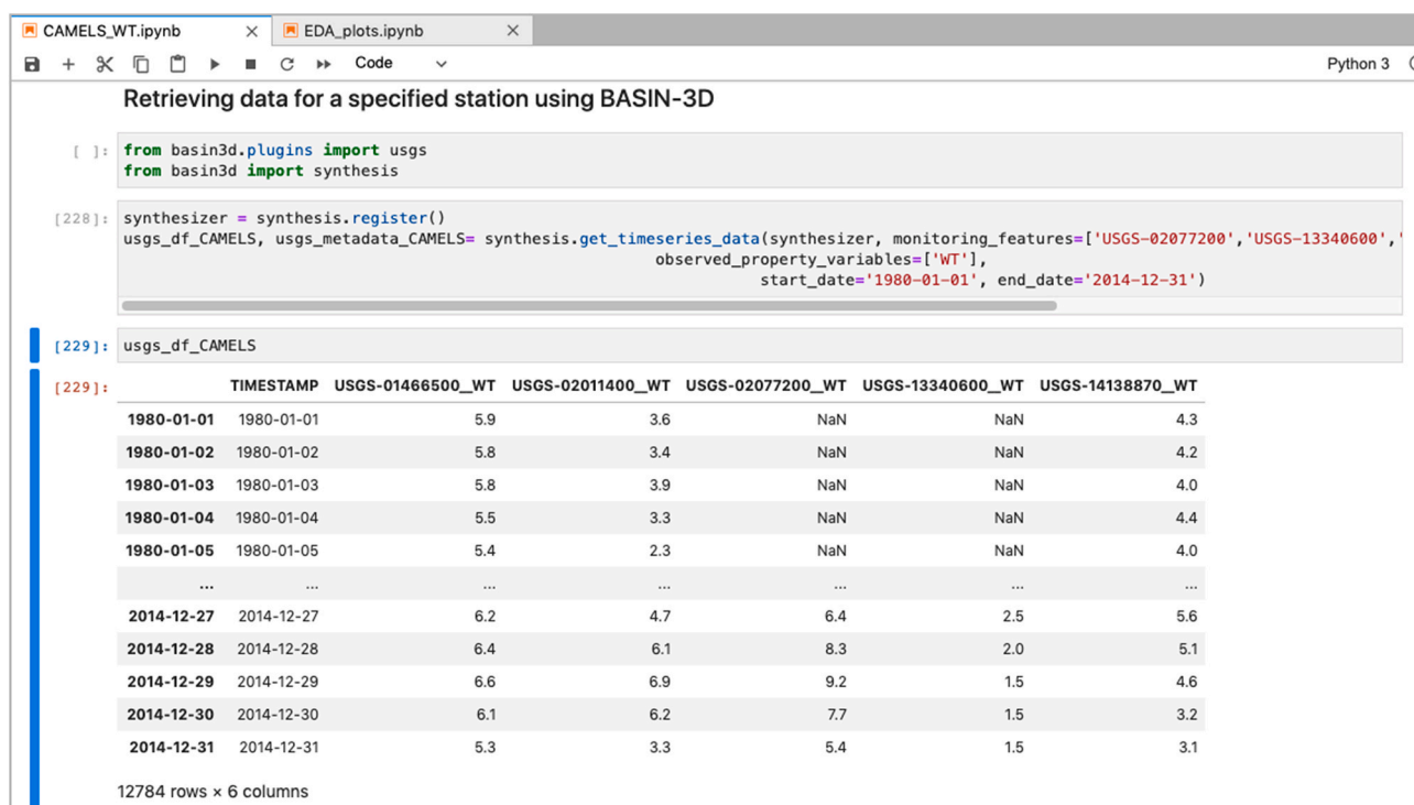
Fig. 4. BASIN-3D can be easily used in a Python-based Jupyter notebook to retrieve synthesized data with a few lines of code.
