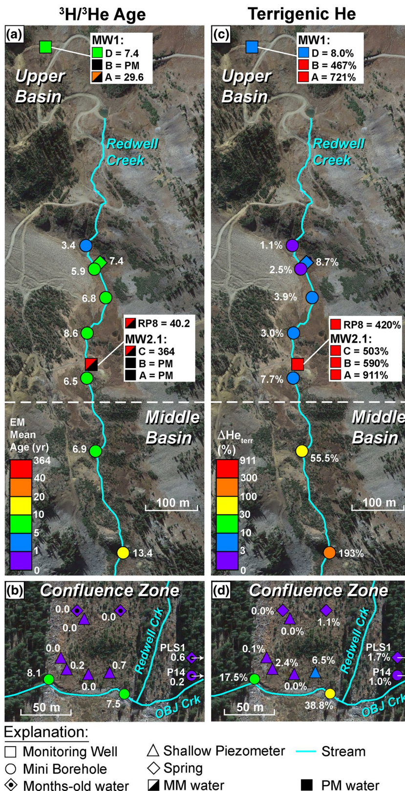
Figure 6. Spatial distribution of ^3\text{H}/^3\text{He} exponential model (EM) mean age in (a) upper and middle basin zones, and (b) confluence zone, along with spatial distribution of terrigenous He ( \Delta\text{He}_{\text{terr}} ) in (c) upper and middle basins, and (d) confluence zone. MM, mixed-modern; PM, premodern; OBJ, Oh-Be-Joyful.
