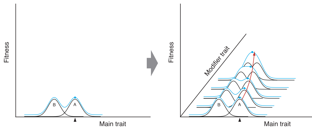
Fig 5. Hypothetical representations of how flowers could adaptively generalize for pollinators through the evolution of two combinational strategies for trade-off mitigation: (A) peak blunting, and (B) optima convergence. Both strategies start from the state where the main trait is adapted to pollinator A (left); because of disruptive selection due to a phenotypic trade-off , these flowers cannot receive contribution from pollinator B. Filled triangles indicate optimal phenotypes. In peak blunting (A; right), as the modifier trait changes, the fitness function of the trait for B is gradually flattened, while that for A hardly changes. This would increase total fitness (blue curves) because flowers can receive marginal benefits from B. In optima convergence (B; right), fitness functions of the trait for A or B (or both) gradually approach each other as the modifier trait changes. This would increase total fitness (blue curves) because they can receive benefits from both pollinators. In both cases, flowers will climb up the fitness ridge (red arrows) through natural selection imposed on the modifier trait.
