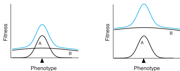
Fig 1. Graphical representations of visitor-mediated phenotypic trade-offs between visitor groups A and B and their possible evolutionary consequences. (A) Fitness function graph showing the relationships between floral phenotype (trait value or status) and the visitor-specific fitness contributions (black curves) as well as the total fitness (blue curve). We refer to the former as visitor-specific fitness functions, and the latter as overall fitness function. (B) Disruptive selection type which produces a distinct phenotype as a singular adaptation to either A or B. Filled triangles indicate optimal floral phenotypes. (C) Stabilizing selection type which produces an intermediate phenotype as a compromise between adaptation to A and B. (D) Unilateral selection type which produces a distinct phenotype as a dual adaptation to both A and B.
