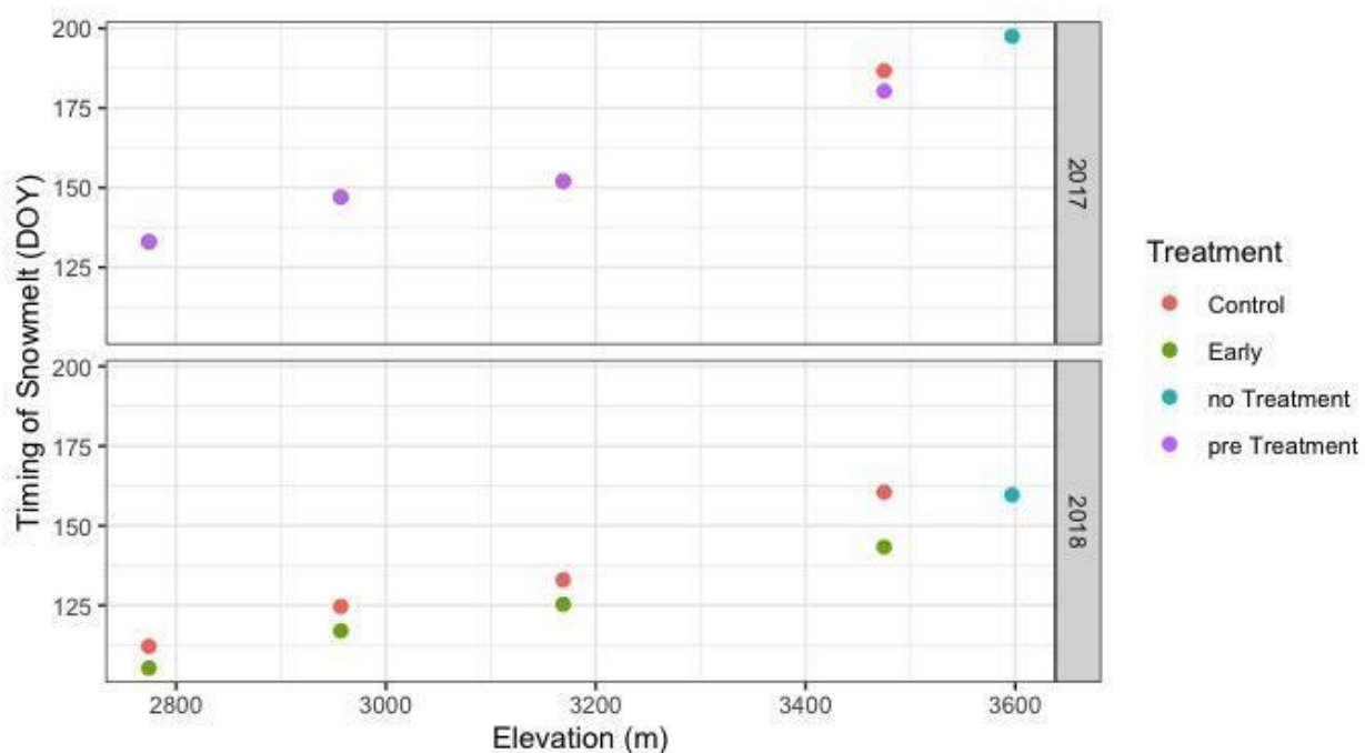
Figure 5. Snowmelt dates in 2017 (no snowmelt manipulation) and 2018 (with snowmelt manipulation). Red dots represent control plots, blue dots represent plots where there was no snowmelt manipulation, purple dots represent pre-treatment plots (designated as a treatment plot before manipulation year), and green dots are plots where there was a snowmelt manipulation. Dates of snowmelt for the lowest three sites in 2017 in 'control' and 'early' plots are the same.
