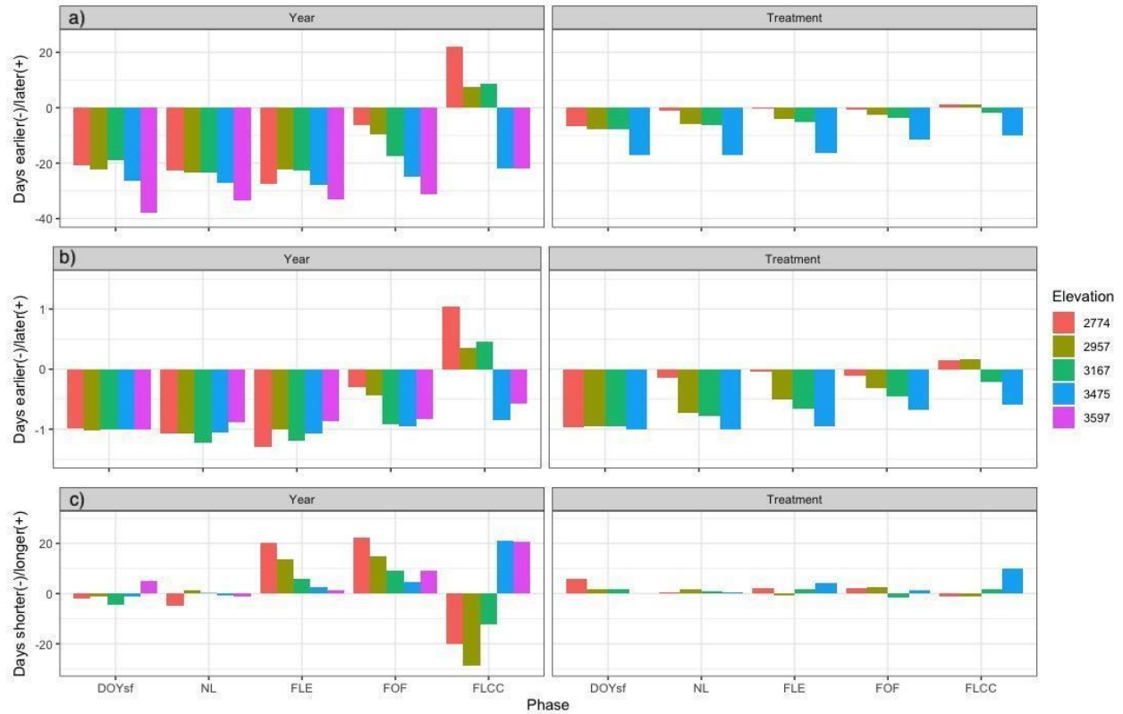
Figure 6. Number of days difference in timing (a and b) and duration (c) for all phenophases at all elevations. Panel a) shows raw statistical results and panel b) shows the statistical results for timing normalized by the number of days advance in day of year snow free (DOYsf). The year effect is calculated as the timing of phenophases in control plots in 2018 - the timing of phenophases in control plots in 2017. The treatment effect is the timing of phenophases in experimentally early plots in 2018 - the timing of phenophases in control plots in 2018.
