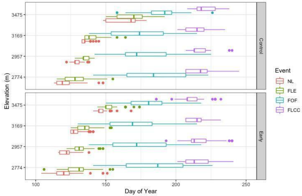
Figure 10. Phenophases in sequence for control and treatment plots in 2018. The start date of each phenophase is the earliest date that was observed for a species at that site. The end date is the last date that the phenophase was observed for a species at that site.
