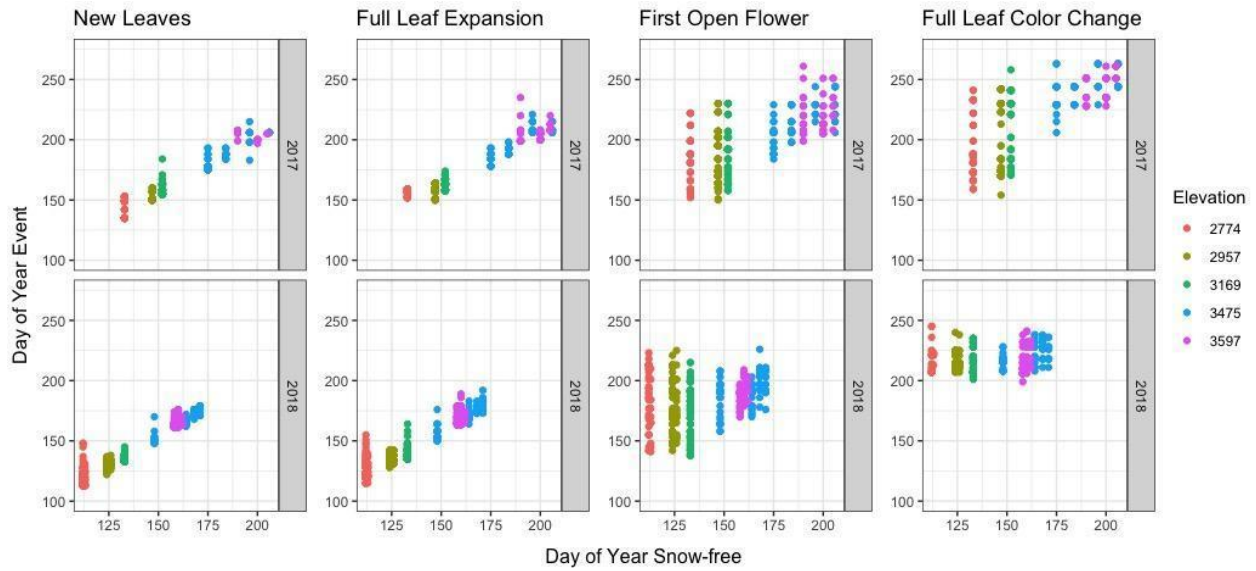
Figure 7. The effect of year on the relationship between the timing of phenophases and the day of year snow free. Data includes control plots in 2017 and 2018.
