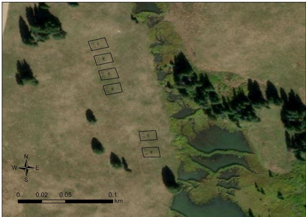
Figure 2. Example plot design. At each site where a snow manipulation was implemented there were six 10mX14m plots paired together into a control and treatment (early) block. Within each larger plot there were two 1mX1m subplots where phenology observations were taken on all species.
