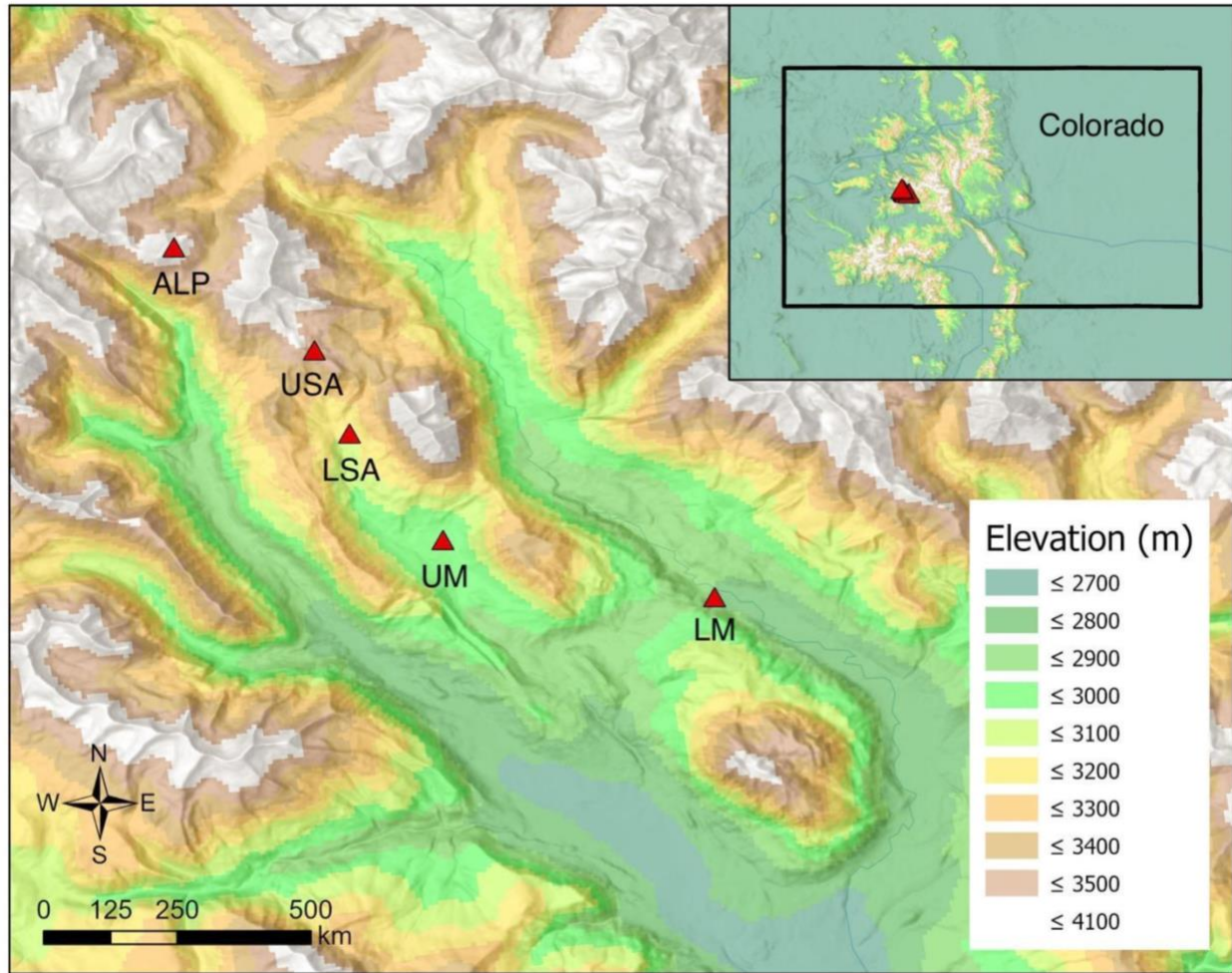
Figure 1. Locations of sites in the East River Valley. From lowest to highest elevation: Lower Montane (LM), Upper Montane (UM), Lower Subalpine (LSA), Upper Subalpine (USA), and Alpine (ALP).
