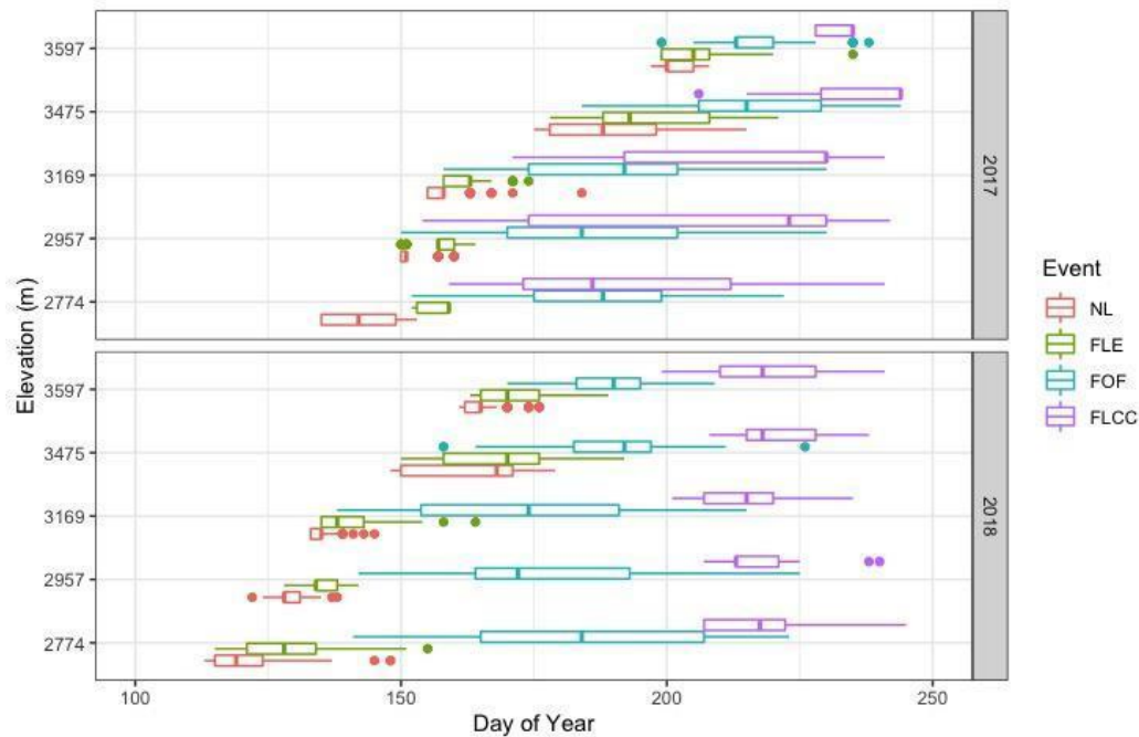
Figure 9. Phenophases in sequence for control plots in 2017 and 2018. The start date of each phenophase is the earliest date that was observed for a species at that site. The end date is the last date that the phenophase was observed for a species at that site.
