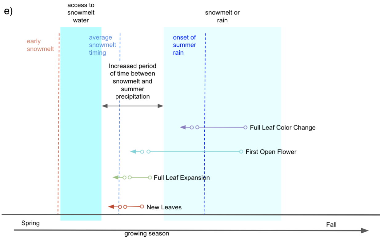
Figure 11. Conceptual diagrams of shifts in water sources and phenophase timing and duration. Panel a) shows a typical growing season where snowmelt water resources and summer rainwater resources are associated with each other. Panel b) shows how shifts in snowmelt timing produces a longer period when the source of water resources is uncertain and could be snowmelt, summer rain, or a lack of water. Panel c) shows shifts in phenophases with early snowmelt and the association of certain phenophases with longer periods of time where water source is not certain. Panel d) shows a situation in which some phenophases' durations are longer and more associated with periods of time when water source is not certain. Panel e) shows a situation in which phenophases do not advance with snowmelt and how this can result in phenophases not being associated with snowmelt water resources.
