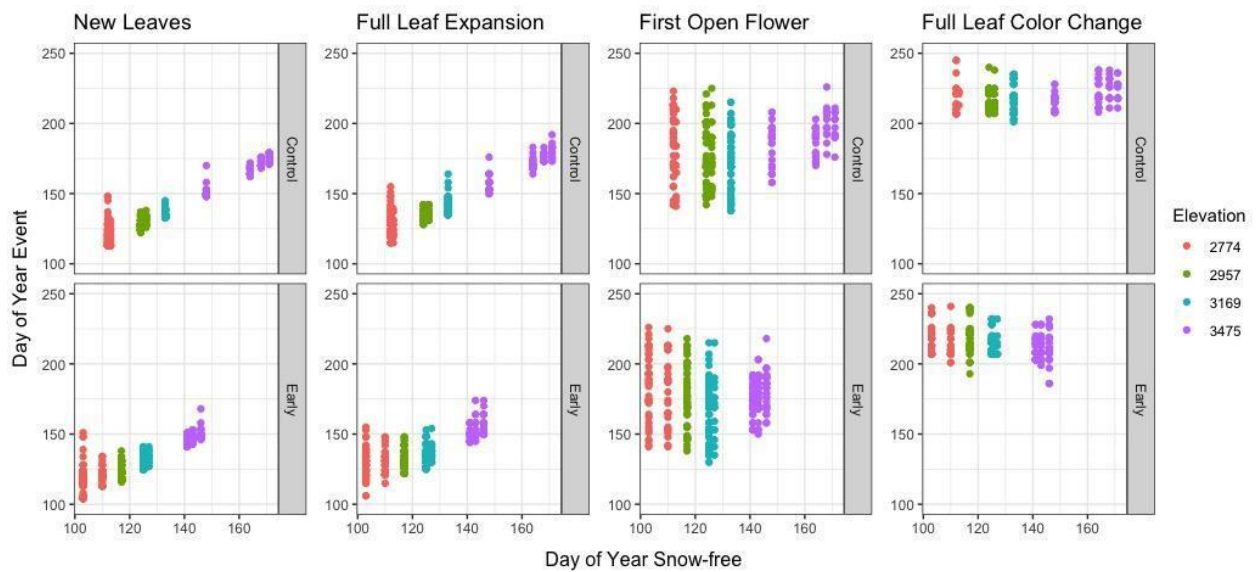
Figure 8. The effect of the treatment on the relationship between the timing of phenophases and the day of year snow free. Data includes control and treatment plots in 2018.
