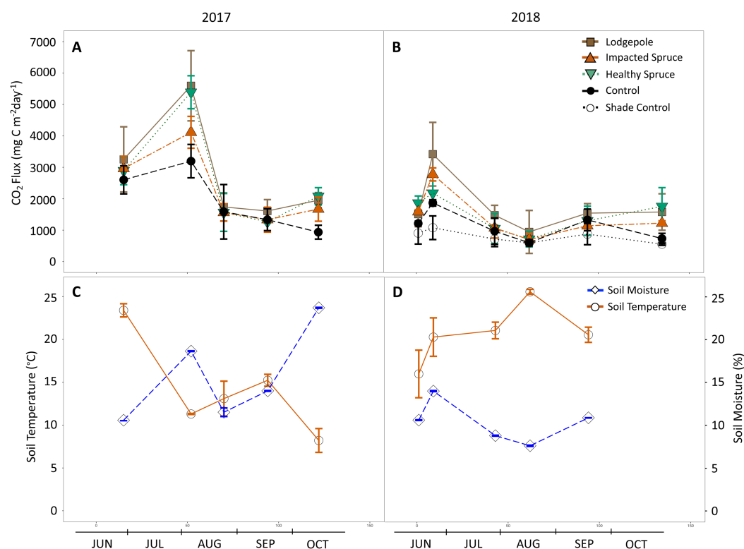
Figure 3 Gas flux as a function of season and needle decomposition. (A and B) Measured carbon dioxide above needle collars and (C and D) on-site soil moisture and temperature during the sampling events of 2017 (A and C) and 2018 (B and D). The gas flux error bars indicate plus or minus one standard deviation ( n = 3 or 4 ). The soil temperature and moisture error bars indicate plus or minus one standard deviation of the hourly values collected during each sampling period. Soil temperature and moisture values are not available for the final date in October 2018. Full-size DOI: 10.7717/peerj.9538/fig-3
