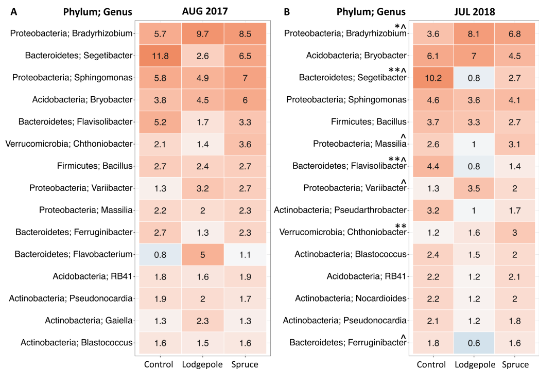
Figure 5 Top 15 most abundant bacterial genera differ as a function of sample type. Top 15 genera in (A) August 2017 and (B) July 2018. Numeric values within each box represent the percent read abundance. Spruce values are binned healthy and impacted spruce ( n = 6 ). Control in July 2018 is binned shaded and non-shaded ( n = 5 ). Mean abundance values are shown within each heatmap box with color representing numerical ranges visually with low values in blue and high values in red. Symbols indicate significant differences determined by differential abundance analysis as follows: ^ Significant difference between lodgepole and controls, * Significant difference between impacted spruce and controls, ** Significant difference between the binned impacted and healthy spruce from the controls.
