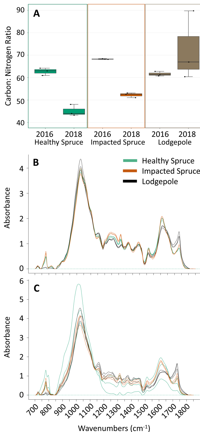
Figure 1 Differences in needle carbon, nitrogen, and organics composition. (A) Percentages of carbon and nitrogen needle composition represented as the carbon:nitrogen ratio ( n = 3 ) for the harvested needles (2016) and after 2 years of decomposition (2018). Points on the plot represent actual values. (B) FTIR spectra for the initial needles and (C) after 2 years of decomposition. Peak heights at specific wavenumbers reveal differences in the spectra as a function of needle species. Total carbon and nitrogen percentages can be found in Table S1. Full-size DOI: 10.7717/peerj.9538/fig-1
