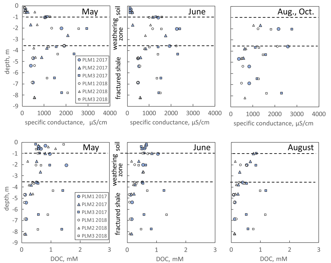
Figure 8. Depth profiles of pore water specific conductance (upper row graphs) and DOC (lower row graphs). The dashed horizontal lines delineate defined boundaries between soil, weathering shale, and fractured shale zones.
