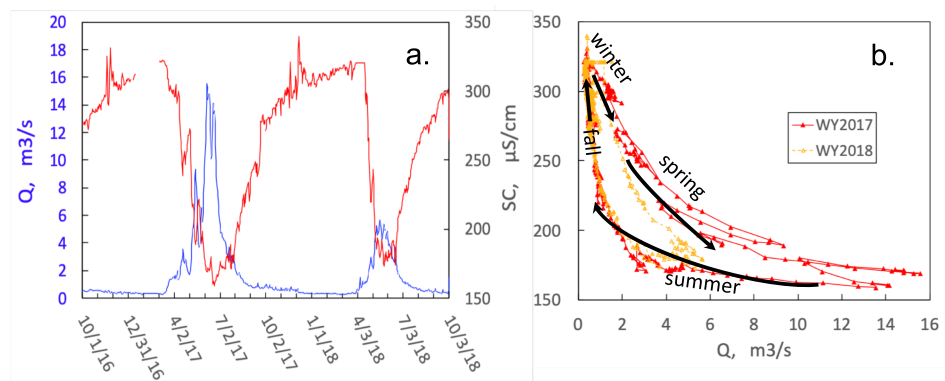
Figure 15. East River discharge and specific conductance at the Pumphouse gauging station. (a) Hydrograph (blue) and SC time trend (red) for WY2017 and WY2018. (b) Q-C relations for SC in the East River.
