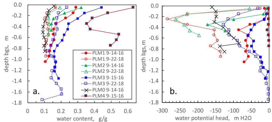
Figure 6. Vertical profiles of (a) soil water content and (b) soil water potential measured on samples collected in September 2016 and 2018.
