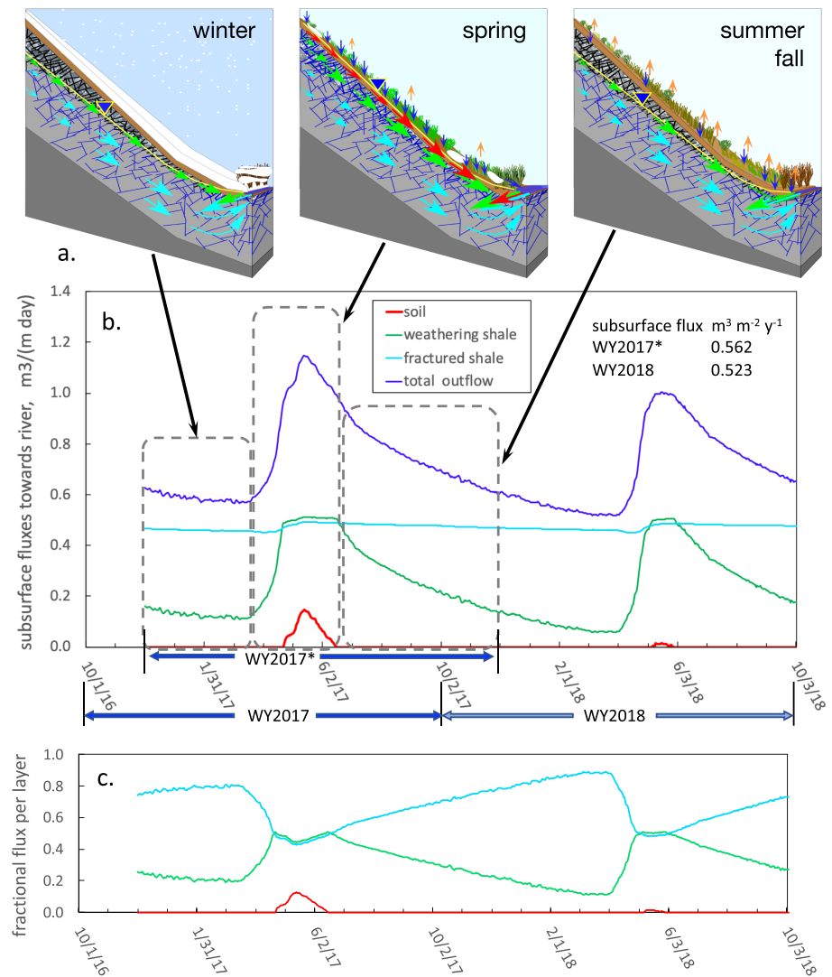
Figure 11. Downslope fluxes from different zones within the hillslope subsurface. (a) Conceptual illustration of annual subsurface fluxes. Saturated downslope flow in the fractured shale, weathering zone, and soil are indicated in turquoise, green and red arrows, respectively. (b) Calculated downslope fluxes through the fractured shale, weathering zone, and soil during WY2017 and WY2018. (c) Time dependence of fractional flow contributions, F_i(t) , from the fractured shale, weathering zone, and soil.
