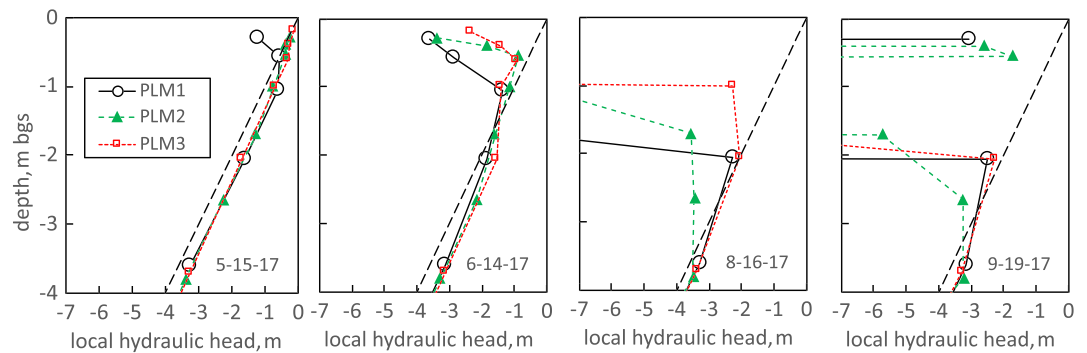
Figure 5. Hydraulic head profiles from the hillslope over the course of 4 months following the WY2017 snowmelt. The gravitational potential datum for each profile is set at its local soil surface, such that the diagonal dashed line represents zero pressure head. The horizontal gray bands indicate locations of the zero-flux boundary (with the uncertainty in depth indicated by shading), above which ET drives net water flux toward the atmosphere.
