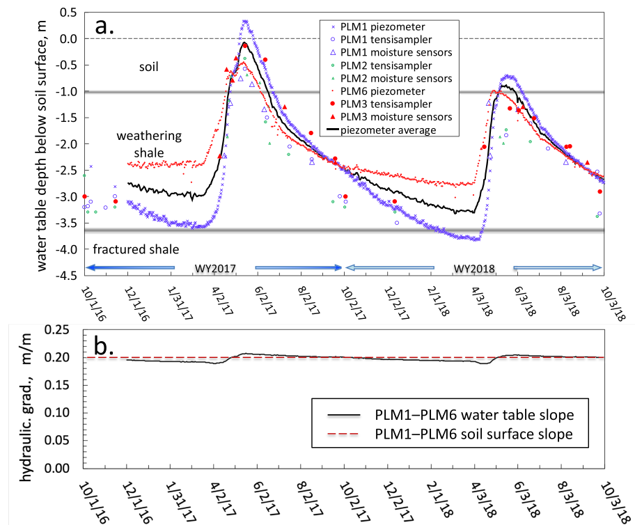
Figure 7. Time trends in the water table along the hillslope transect during WY2017 and WY2018. (a) Depths to the water table determined with piezometers, and estimated with tensisamplers and moisture sensors. The heavy black line is the average of PLM1 and PLM6 piezometers, used in transmissivity feedback calculations. (b) Comparison between the water table slope and the average soil surface slope ( 0.200 \text{ m m}^{-1} ) along the transect.
