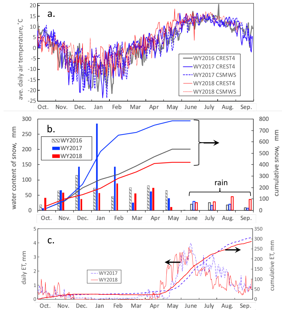
Figure 2. Weather data and calculated ET for the study area. (a) Daily average air temperatures from weather stations located 0.3 km (CSMWS) and 5.3 km (CREST4, at Gothic, CO) away from the transect. The CREST4 station (recording weather data since 1974) is located near the East River, at an elevation of about 2,910 m (similar to that of our upper hillslope). (b) Monthly water content of snow and monsoon rainfall (CREST4). (c) Daily and cumulative ET calculated with the CML (Tran et al., 2019).
