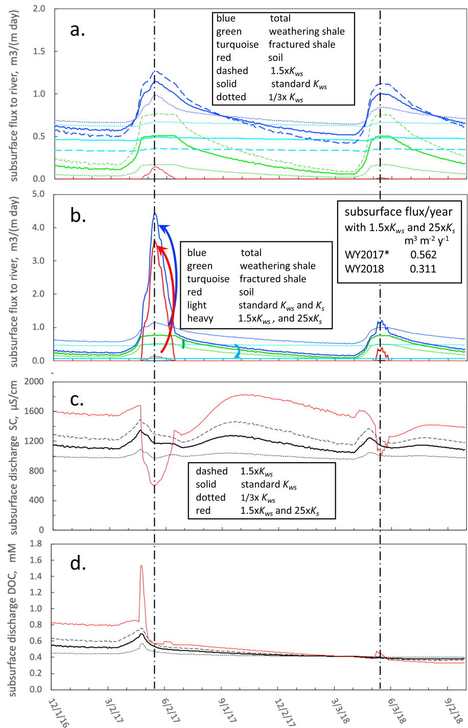
Figure 14. Impacts of different K values on the predicted water fluxes, discharge SC, and discharge DOC. Time trends for (a) influences of different K_{ws} on subsurface fluxes within different zones, (b) influences of increasing both K_s and K_{ws} on subsurface fluxes within different zones, (c) subsurface flow-weighted SC of discharging pore waters, and (d) subsurface flow-weighted DOC concentrations in discharging pore waters. The K for fractured shale bedrock was kept constant, while the thickness of the fractured shale was adjusted to achieve water mass balance. Vertical dashed lines indicate dates associated with calculated annual peak subsurface discharge rates.
