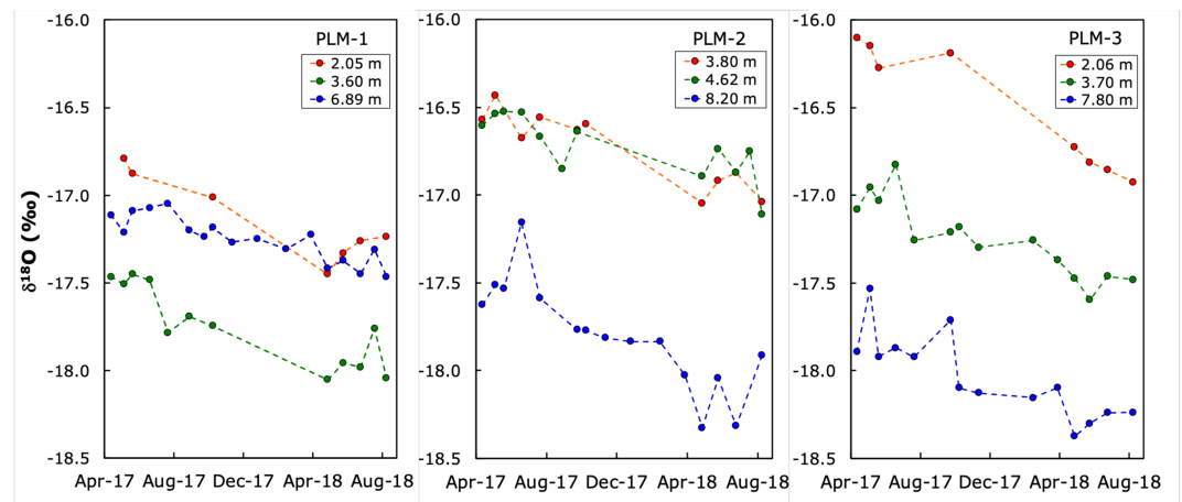
Figure 10. Time trends in \delta^{18}\text{O} of depth-resolved groundwaters from the three hillslope monitoring stations.
