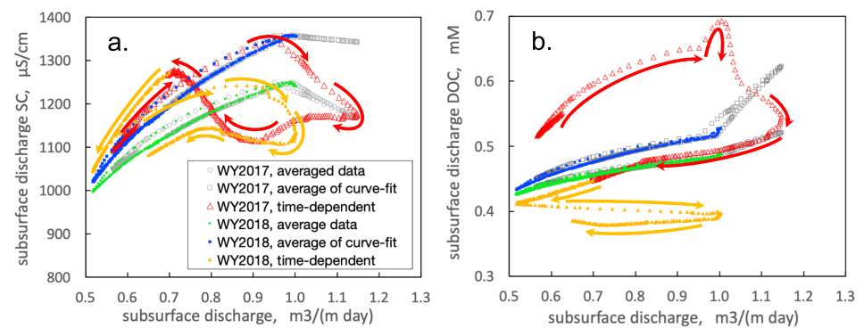
Figure 13. Hillslope subsurface concentration-discharge relations for (a) specific conductance and (b) dissolved organic carbon. Arrows along the time-dependent curves indicate the direction of time.
