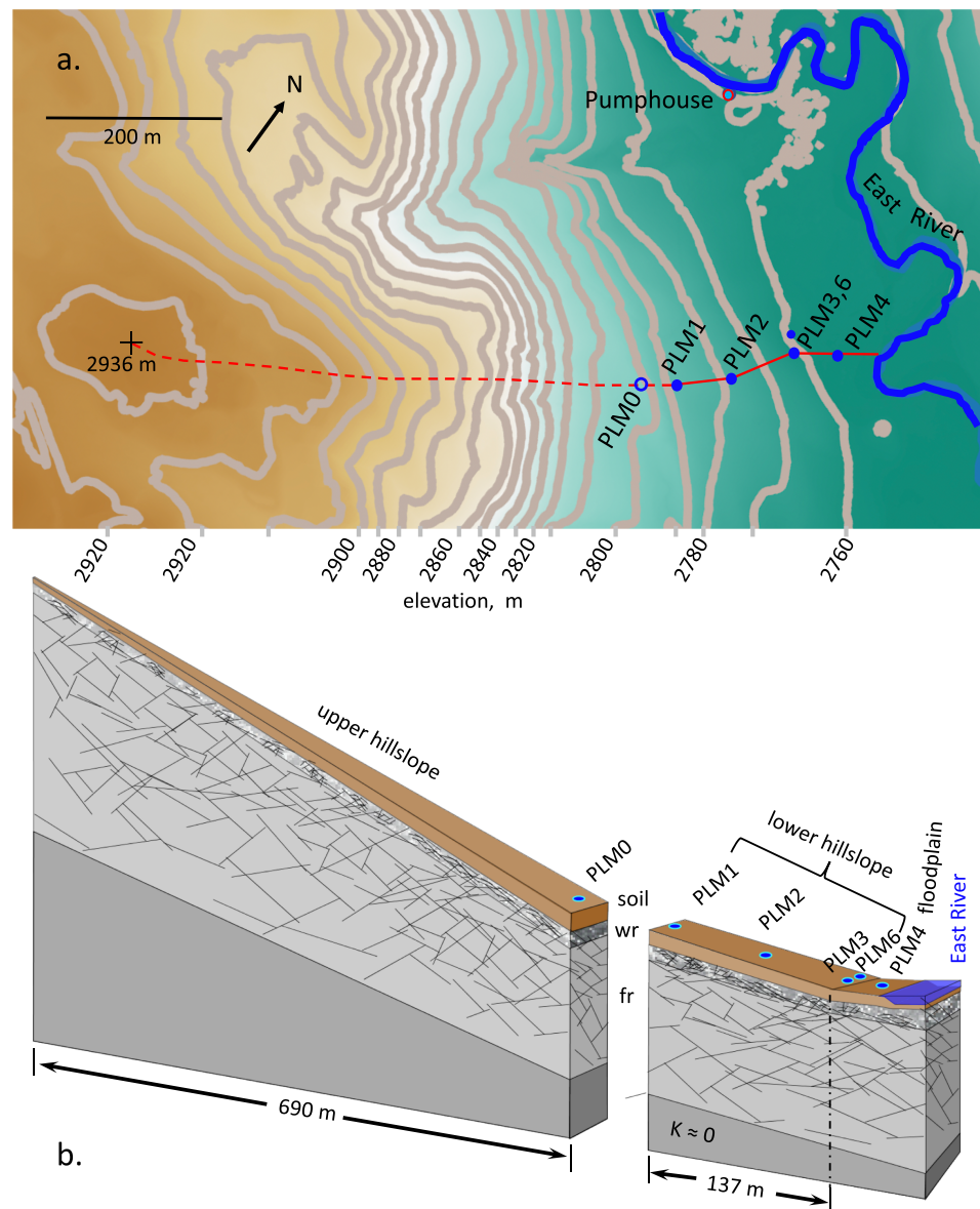
Figure 1. (a) Topographic map showing the PLM transect and upper hillslope region. (b) Conceptual model of the flow domain showing the upper hillslope, monitored lower hillslope, and floodplain, with the subsurface compartmentalized into soil, weathering rock (wr), and fractured rock (fr), underlain by an effectively impermeable lower boundary at a depth to be estimated.
