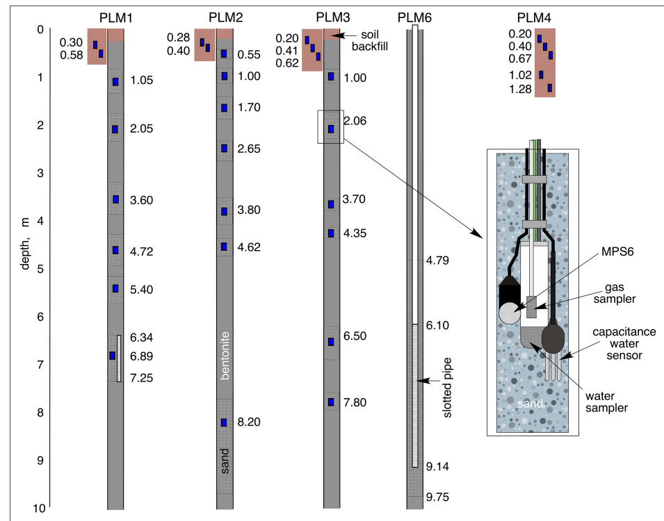
Figure 3. Depth distribution of monitoring and sampling devices in boreholes and wells. Depths of instrument clusters are indicated by blue rectangles in borehole profiles.
