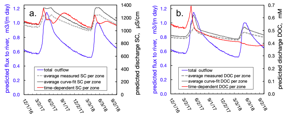
Figure 12. Time trends in predicted subsurface fluxes and discharge concentrations for (a) SC and (b) DOC.
