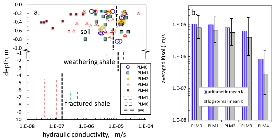
Figure 4. Compilation of hydraulic conductivity values measured along the hillslope and floodplain. (a) Depth distributions of measurements at different stations. The vertical dashed black lines indicate the representative K values for the soil, weathering shale, and fractured shale zones, used in estimates of hillslope subsurface flow. Note that the floodplain soils at PLM4 were not used for estimating the average hillslope soil K . (b) Averages of K values obtained in soils at each station.
