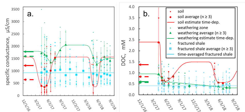
Figure 9. Time trends in pore water specific conductance (a) and DOC (b). The analyses of PLM1–3 pore waters are grouped into three zones; soil (to 1.00 m depth), weathering zone (1.00 to 3.60 m), and fractured shale (deeper than 3.60 m). Horizontal arrows along the vertical scales indicate average values of data (dashed) and curve-fit trends (solid) for the soil (red) and weathering zones (green), respectively.
