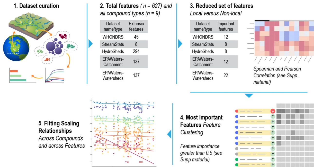
Fig. 3. Scaling methodology: Step 1: Dataset curation, including collecting all data and conducting QA/QC on all data. Step 2: Aggregating all data to the correct scales and co-locating watershed data with DOM data. Step 3: Reducing the number of features using six different sensitivity methods (i.e., Spearman's correlation, Pearson correlation, F-test, Mutual information, Feature importance based on Random Forests, and SHAPley values) to reduce bias in selecting key features for developing scaling laws 56,58 . Step 4: Feature selection using feature clustering. Any feature importance greater than 0.5 constitutes a behavioural set for which feature importance values are deemed to satisfy user-defined performance metrics (e.g., averaged importance values greater than 0.5 across multiple sensitivity analysis methods to reduce any bias in selecting variables for developing scaling laws) 59,60 . Step 5: Fitting scaling relationships to compound class and most important features.
