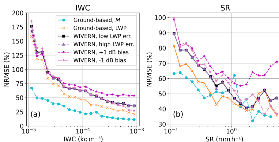
Figure 10. Normalized root mean square error (NRMSE) in percentage as a function of ground-based and space-borne (WIVERN) estimates of (a) IWC and (b) SR, respectively. NRMSEs for positive and negative bias in Z_e of 1 dB are shown in magenta and pink, respectively. Note the different y axis scales.
