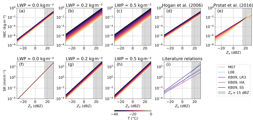
Figure 5. IWC– Z_e (a–e) and SR– Z_e (f–i) empirical functions for (a, f) \text{LWP} = 0.0 \text{ kg m}^{-2} , (b, g) 0.2 \text{ kg m}^{-2} , and (c, h) 0.5 \text{ kg m}^{-2} and T ranging from -40^{\circ}\text{C} to 0^{\circ}\text{C} . Empirical IWC– Z_e functions from Hogan et al. (2006) and Protat et al. (2016) are shown in (d) and (e), respectively. SR– Z_e values from Matrosov (2007) (M07), Liu (2008) (L08), and Kulie and Bennartz (2009) (KB09, LR3; KB09, HA; KB09, SS) are shown in (i). Due to data availability, Z_e > 15 \text{ dBZ} is shaded in black.
