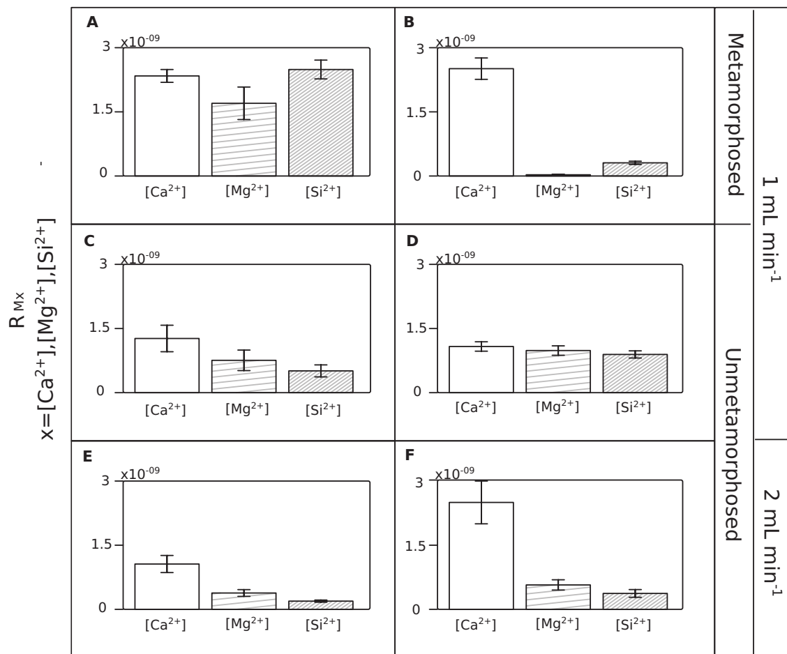
Figure 2.4. Summary figure showing average steady state mass normalized release rates for all columns at all flow conditions. Metamorphosed samples UM1A and UM1B are shown on the top row in subfigures A and B respectively. Samples UU and WU at 1 \text{ mL min}^{-1} are shown in C and D respectively, with UU2 and WU2 at 2 \text{ mL min}^{-1} shown in subfigures E and F.
