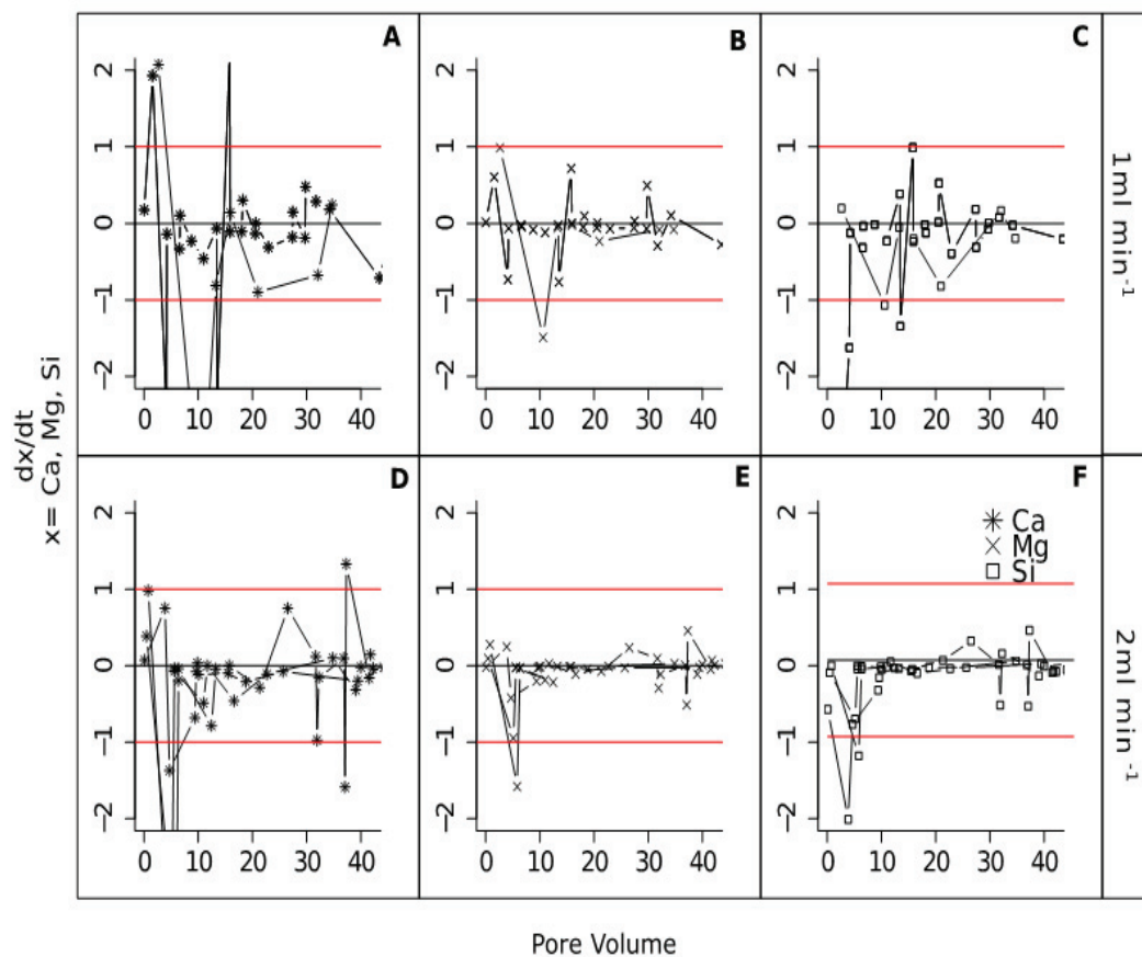
Figure 2.3. Steady state estimations for all trials of unweathered unmetamorphosed UU at 1 mL min -1 (A, B and C respectively) and at 2 mL min -1 (D, E and F respectively). Steady state change in concentration in mg/L for Calcium, Magnesium and Silica are reported for each UU sample at each flow condition.
