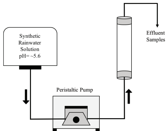
Figure 2.2. Schematic of the flow-through column scale experimental set up for studying solute release rates as a function of mineralogy and degree of metamorphism.
