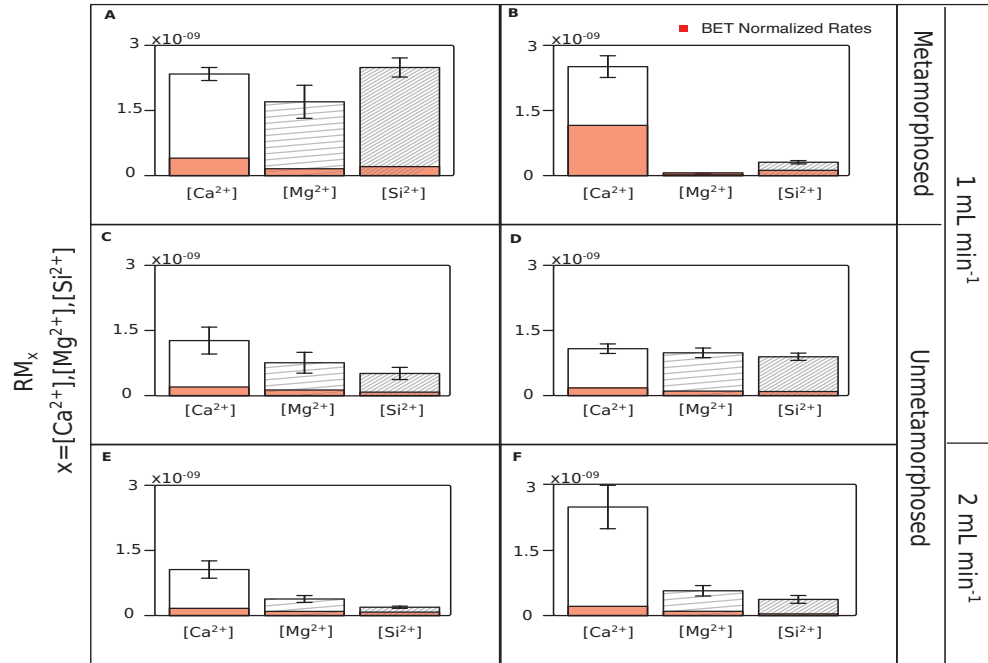
Figure 2.5. A comparison of mass normalized and BET normalized steady state release rates for Ca, Mg, Si.
